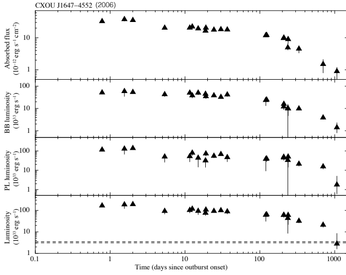
Figure D5. Left-hand panel: temporal evolution of the fluxes and luminosities for the BB+PL model applied to the X-ray data of CXOU J164710.2–455216. The dashed lines mark the 1\sigma c.i. range for the quiescent luminosity (see Table 4). A distance of 4 kpc was assumed. Right-hand panel: temporal evolution of the bolometric luminosity with the best-fitting decay model superimposed.
