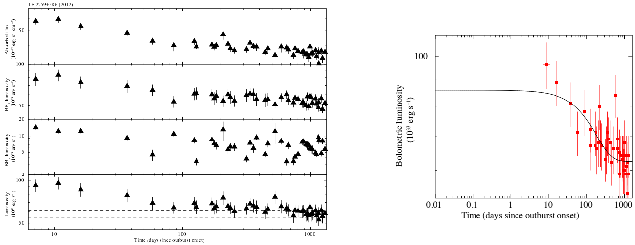
Figure D16. Left-hand panel: temporal evolution of the fluxes and luminosities for the 2BB model applied to the Swift data of the 2012 outburst of 1E 2259+586. The dashed lines mark the 1\sigma c.l. range for the quiescent luminosity (see Table 4). energy range. A distance of 3.2 kpc was assumed. Right-hand panel: temporal evolution of the bolometric luminosity with the best-fitting decay model superimposed.
