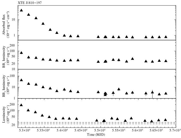
Figure D3. Left-hand panel: temporal evolution of the fluxes and luminosities of the cold and warm blackbody components for the 3BB+2BB model applied to the XMM-Newton data of the 2003 outburst of XTE J1810–197. The dashed lines mark the 1\sigma c.l. range for the quiescent luminosity (see Table 4). A distance of 3.5 kpc was assumed. Right-hand panel: temporal evolution of the bolometric luminosity with the best-fitting decay model superimposed.
