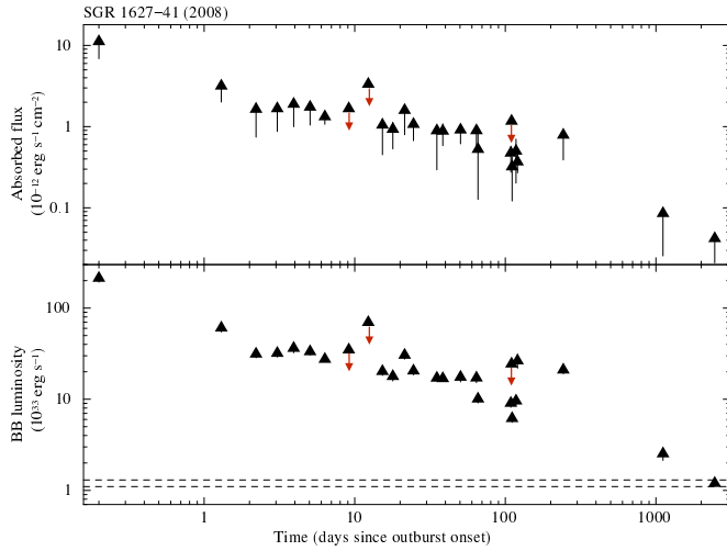
Figure D6. Left-hand panel: temporal evolution of the fluxes and luminosities for the BB model applied to the X-ray data of the 2008 outburst of SGR 1627–41. The dashed lines mark the 1\sigma c.i. range for the quiescent luminosity (see Table 4). The red downward arrowheads indicate the 3\sigma upper limits. A distance of 11 kpc was assumed. Right-hand panel: temporal evolution of the bolometric luminosity with the best-fitting decay model superimposed.
