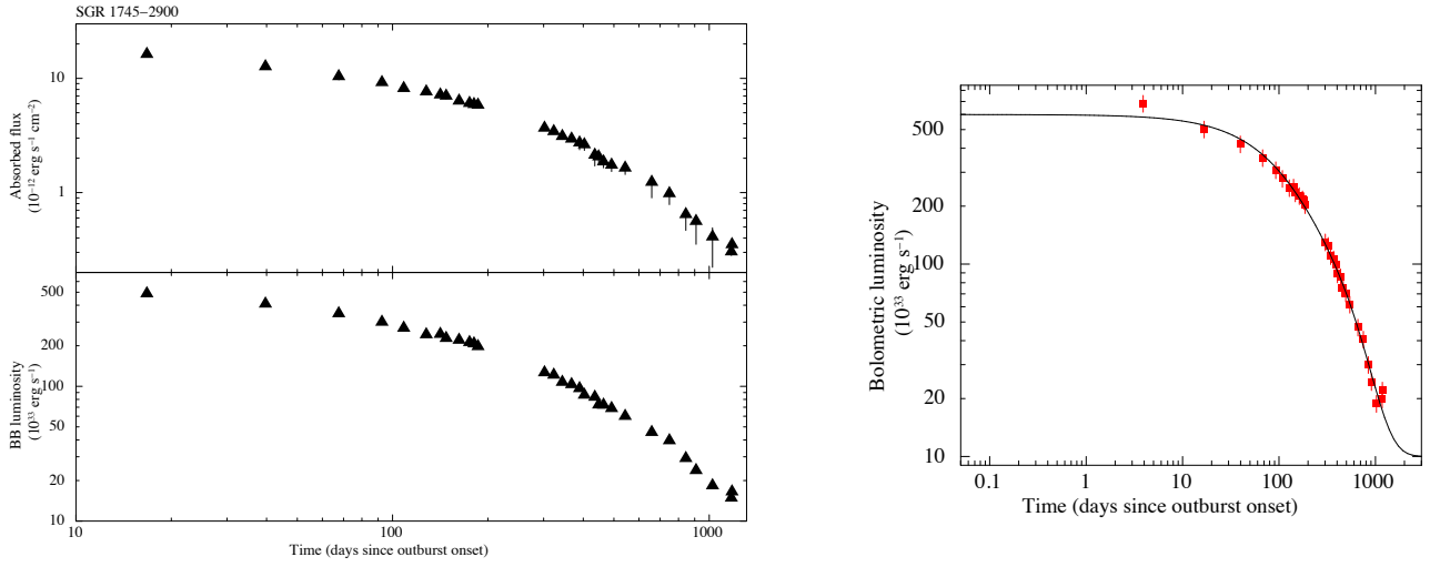
Figure D17. Left-hand panel: temporal evolution of the fluxes and luminosities for the BB+PL model applied to the Chandra data of the outburst of SGR 1745–2900. A distance of 8.3 kpc was assumed. Right-hand panel: temporal evolution of the bolometric luminosity with the best-fitting decay model superimposed.
