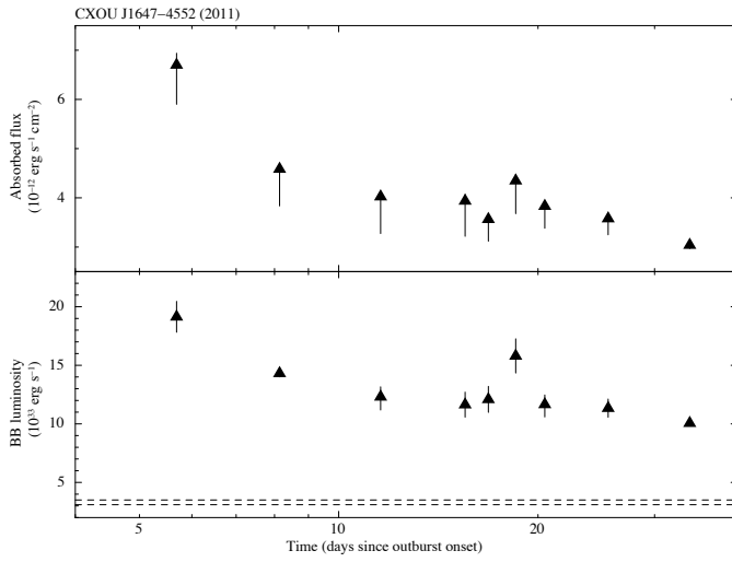
Figure D14. Left-hand panel: temporal evolution of the fluxes and luminosities for the BB model applied to the X-ray data of the 2011 outburst of CXOU J164710.2–455216. The dashed lines mark the 1\sigma c.l. range for the quiescent luminosity (see Table 4). A distance of 4 kpc was assumed. Right-hand panel: temporal evolution of the bolometric luminosity with the best-fitting decay model superimposed.
