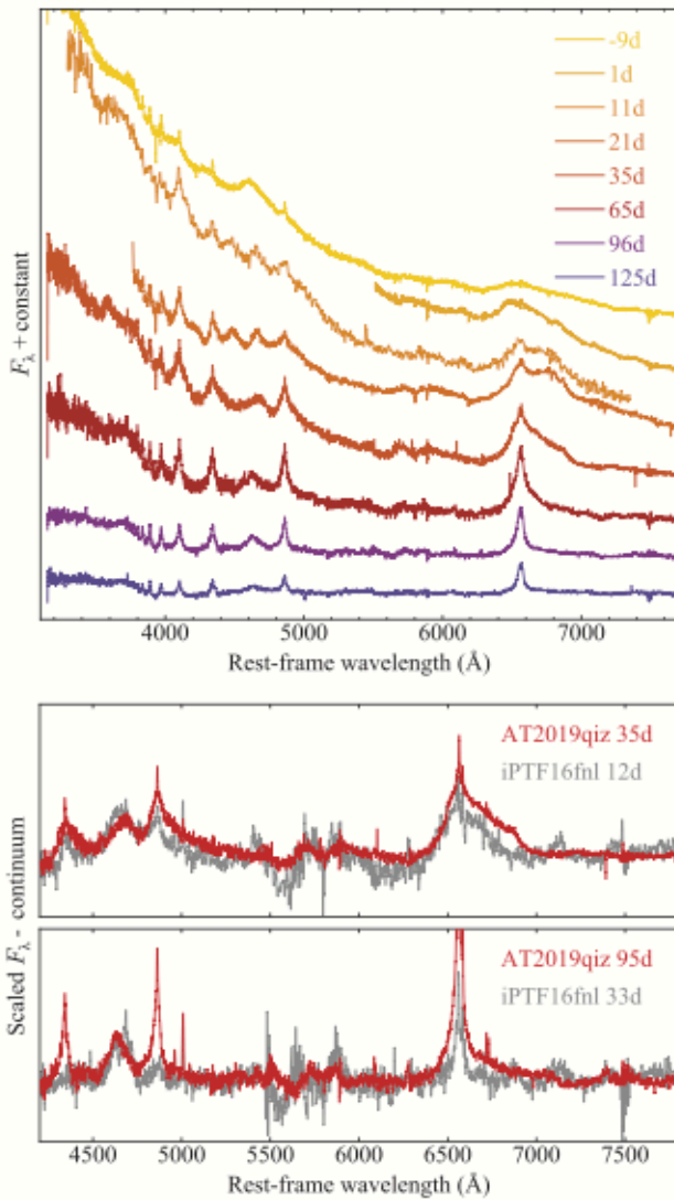
Figure 13. Top: selected spectra from X-shooter, EFOSC2, and Binospec after subtraction of the host galaxy model (following the method outlined in the appendix). We have applied the subtraction procedure to all spectra, but here show only this subset (spanning the full range of observed phases) for clarity. Bottom: Comparison of AT2019qiz to X-shooter spectra of iPTF16fnl (from Onori et al. 2019), the only TDE with a faster light-curve evolution than AT2019qiz. The continuum has been removed using polynomial fits. The spectra shortly after maximum light are quite similar for these two events, though the Balmer lines are much weaker at late times in iPTF16fnl.
