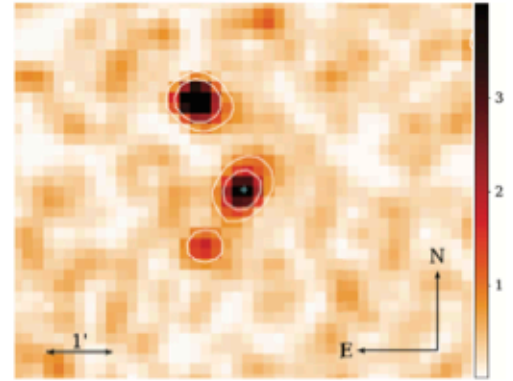
Figure 3. Stacked Swift XRT image (total exposure time 30 ks) centred at the position of AT2019qiz, marked by a cyan cross. An X-ray source is detected at 5.6\sigma significance. The image has been blocked 4 \times 4 and smoothed using a Gaussian kernel for display. The colour bar gives the counts per pixel.
