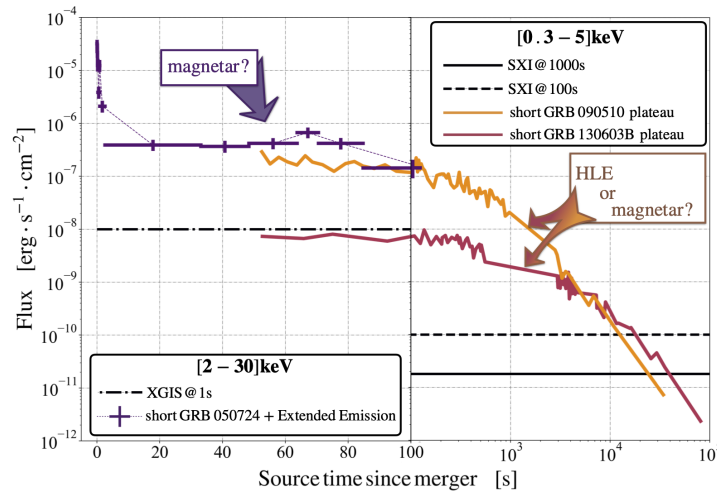
Figure 5. The X-raylong monitoring from prompt emission to the afterglow of relatively bright short GRB with THESEUS/XGIS and SXI. The linear temporal-scale plot on the left shows the short GRB prompt with the “Extended Emission” as it would be detected by THESEUS/XGIS possibly explained by invoking a magnetar remnant. The logarithmic temporal-scale plot on the right shows the X-ray plateau phase with the indication of two possible scenarios invoked for its origin, i.e., High-Latitude Emission of the prompt assuming a structured jet [22] and a spinning-down magnetar pumping energy into the external shock [37] [Credit: S. Vinciguerra].
