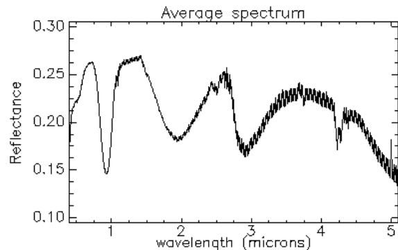
Figure 2: VIS-IR average reflectance spectrum of GRO95535 powder
