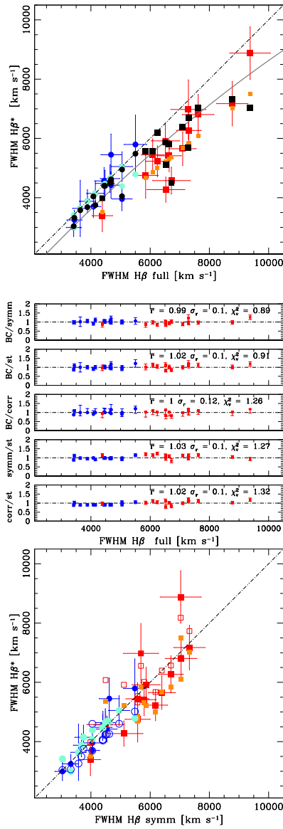
Fig. 2. Virial broadening estimators based on \text{H}\beta , with several corrections applied to the HE sample. Top square panel: \text{FWHM H}\beta_{\text{BC}} (blue (Pop. A) and red (Pop. B)) with error bars, symmetrized \text{FWHM H}\beta (symm, black), and \text{FWHM H}\beta corrected according to spectral type (st, aquamarine and dark orange for Pop. A and B respectively) versus \text{FWHM} of the full \text{H}\beta profile. The grey line traces the correction (corr) following the relation of Sulentic et al. (2006b) reported in §4. Middle panels: ratios of \text{FWHM} after various corrections vs. full profile \text{FWHM} . First panel from top: \text{BC/symm} , \text{BC/st} , \text{BC/corr} , \text{symm/st} , \text{corr/st} . Average values, standard deviation and normalized \chi^2_{\nu} are reported in the upper right corner of the panels. Bottom square panel: BC, spectral type st and reverberation corrected (corr, open symbols) \text{FWHM} values vs. symmetrized \text{FWHM} .
