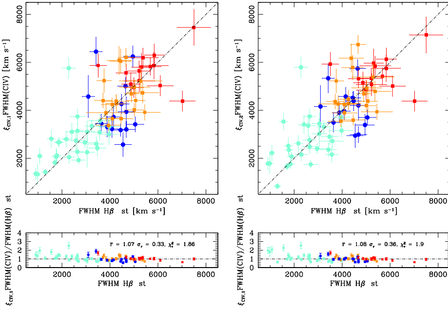
Fig. 7. Top left panel: \xi_{\text{CIV}}\text{FWHM}(\text{Civ}\lambda 1549) i.e., \text{FWHM}(\text{Civ}\lambda 1549) after correction for blueshift and luminosity dependence following Eq. 6 vs \text{FWHM}(\text{H}\beta) cm for the FOS+HE sample. The black dot dashed line is the equality line, meaning of color code is the same as in Fig. 3. Top right: same, but with \xi_{\text{CIV}} computed from Eq. 7.
