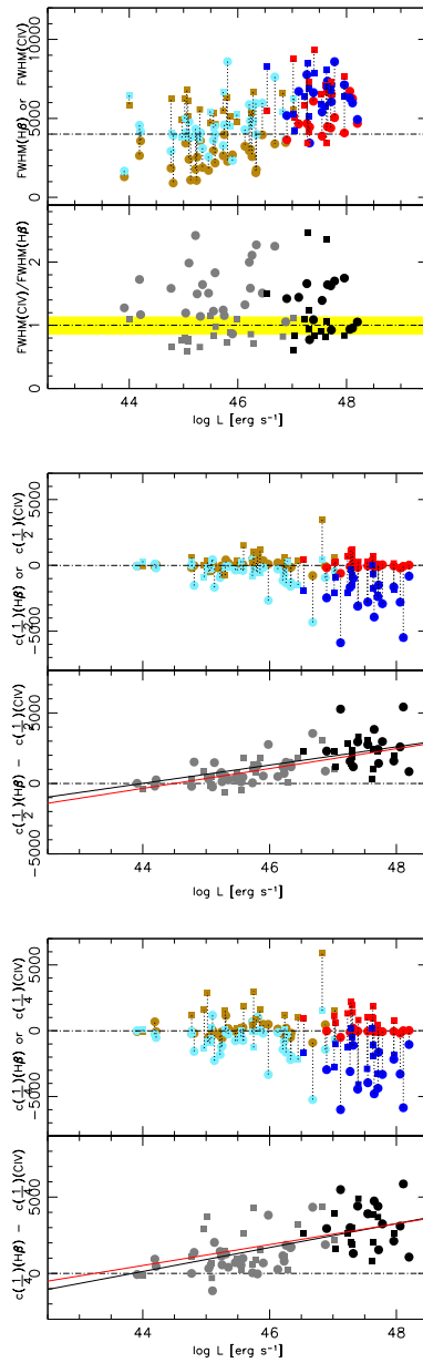
Fig. 9. H \beta and C \nu\lambda 1549 profile parameter comparison as a function of luminosity. Top panels: behavior of FWHM C \nu\lambda 1549 and H \beta (upper half) and of the ratio FWHM(C \nu\lambda 1549 )/FWHM(H \beta ) as a function of L (lower half), for FOS (golden and pale blue) and HE sample (red and blue). The yellow band identifies the region where FWHM(C \nu\lambda 1549 )/FWHM(H \beta )=1 within the errors. Middle panels: c(\frac{1}{2}) of H \beta and C \nu\lambda 1549 (upper half), and difference \delta(\frac{1}{2}) as a function of L (lower half). Square symbols indicate Pop. B, circles Pop. A. Lines trace an unweighted lsq fit for the Pop. A (black) and for Pop. B (red) sources. Bottom panels: same for c(\frac{1}{4}) and \delta(\frac{1}{4}) . The vertical dotted lines join H \beta and C \nu\lambda 1549 parameters for the same object (e.g., they are not error bars).
