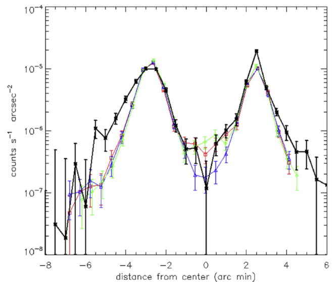
Figure 10. X-ray surface brightness profiles along the line connecting the two X-ray peaks from Chandra observations (stars with error bars connected with thick black solid lines), from mock observations with V_{\text{infall}} = 1000 and 2000 \text{ km s}^{-1} (red squares and green diamonds with error bars connected with solid lines of the same color; presented in Figure 9), and from mock observations assuming that the clusters are not interacting, they look close to each other only in projection (blue triangles with error bars).
