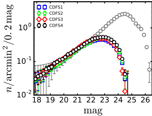
Figure 1. The r -band magnitude distributions with errorbars estimated from the Poisson statistics. The grey points represent the distribution of the det image, while the other four color-encoded distributions are the results by averaging the individual catalogs of all epochs for the sub-fields, respectively.
