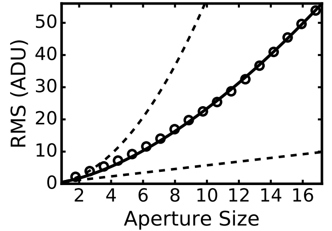
Figure 6. Gaussian dispersion as a function of aperture size defined as \sqrt{N} . The black circles are measured from the difference image D_I . A power-law curve with free parameter \beta (solid line) is used to fit the data points. For illustration, the bottom and top dashed curves represent two limiting cases: no pixel correlation and complete correlation in adjacent pixels.
