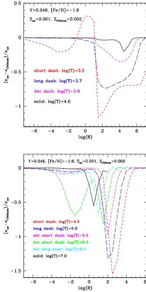
Fig. 2 Relative difference of the radiative Rosseland mean opacity between a standard P1 \alpha -enhanced composition, and the CNO-enhanced P2 CNO_{enh} composition at fixed [Fe/H] and Y , and several temperatures (see labels), as a function of the density parameter R (see text for details). The corresponding total metal mass fractions Z are also labelled.
