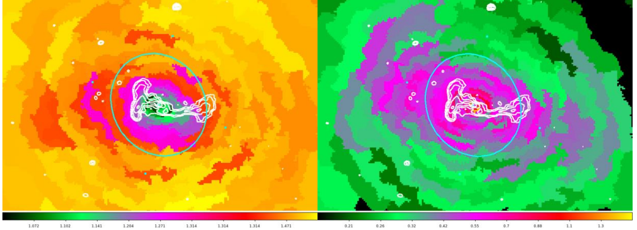
Figure 6. GMRT 610 MHz radio contours (from Kolokythas et al. 2020) showing the AGN jets and lobes are overlaid on the T map (left) and the Fe map (right). The cyan ellipse indicates the D_{25} ellipse.
