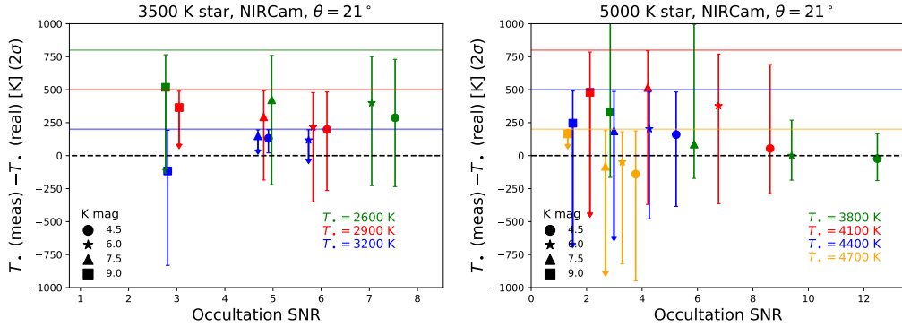
Figure 7. Same as Figure 5 for spots at 21° stellar latitude, for the M (left) and K (right) scenarios observed by NIRCam/F150W2 + F322W2.
