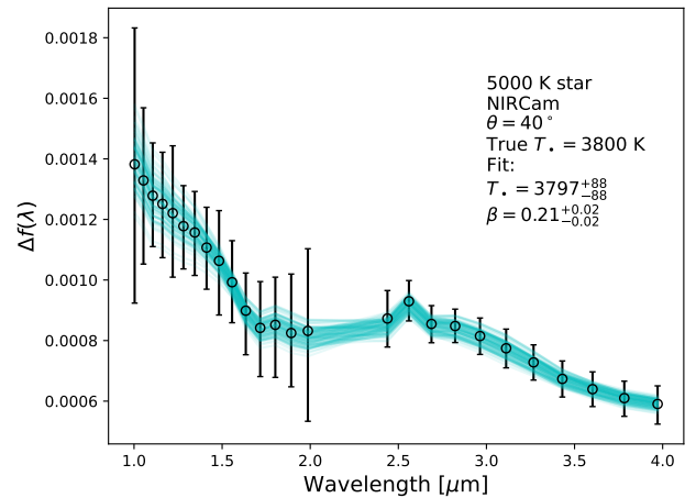
Figure 4. Example of in-transit starspot crossing flux bumps measured with the model in Equation 8 and their uncertainties, for the \text{mag}_K = 7.5 , K star case, in the T_* = 3800 K, \mu -angle \theta = 40^\circ scenario without in-transit Gaussian scatter. The models in light blue represent 100 fitting models sampled from the T_* and \beta posterior distributions. The result of the nested sampling for fitted parameters, and their 68% credible intervals, are indicated in the label. The model spectra were convolved with the NIRCam filters and degraded to the same resolutions as the observations before performing the fit.
