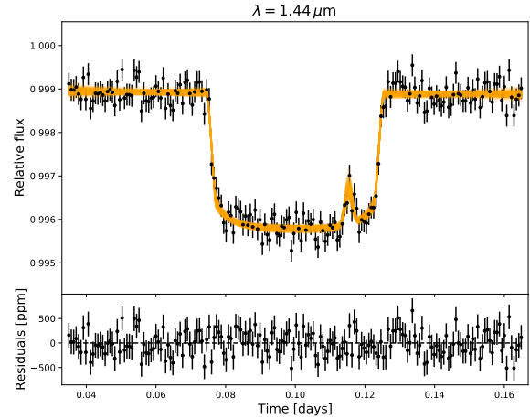
Figure 3. Simulated transit of a 0.25 R_J planet orbiting a 10.5\text{-mag}_K , 0.47 R_\odot , 3500 K star, occulting a 2900 K starspot at limb angle \theta = 40^\circ , observed with NIRSpec/Prism in the wavelength bin centred at \approx 1.4 \mu\text{m} . This plot presents one of the noise realisations to better show the extent of the flux uncertainties. In orange on the upper panel, 300 samples from the posterior distributions obtained with the transit and Gaussian profile modelling are shown. The lower panel shows the residuals of the best-fit model, presenting a white-noise scatter, in parts per million.
