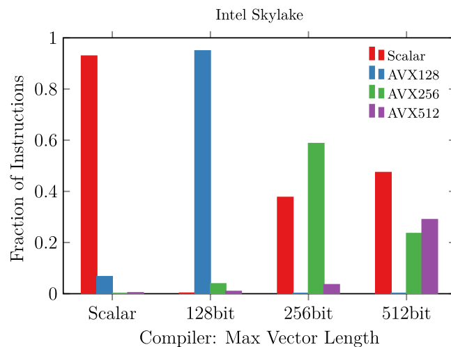
Figure 35. Fractional number of instructions generated by the Cray compiler over the limit of the vector length. Top for Intel Broadwell, bottom for Intel Skylake.
