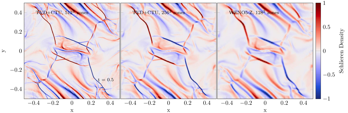
Figure 17. Schlieren image of the density in the Orszag–Tang vortex test at t = 0.5 for TVD+CTU with 512^2 zones (left) and 256^2 zones (middle), and WENO5-Z with 128^2 zones (right).
