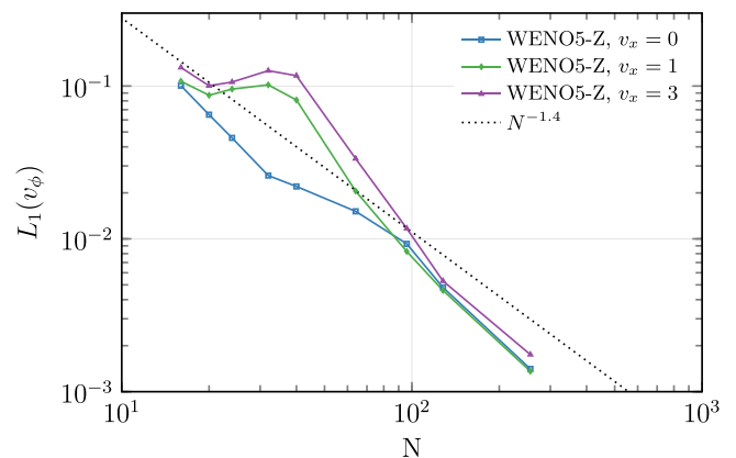
Figure 23. L_1 error norm of the angular velocity v_\phi in the Gresho vortex test at t = 3 for three WENO5 simulations with v_x = 0 (blue), v_x = 1 (green), and v_x = 3 (purple). The dotted line corresponds to a scaling of N^{-1.4} and is normalized to approximately correspond to the results shown in Springel (2010), their Figure 29.
