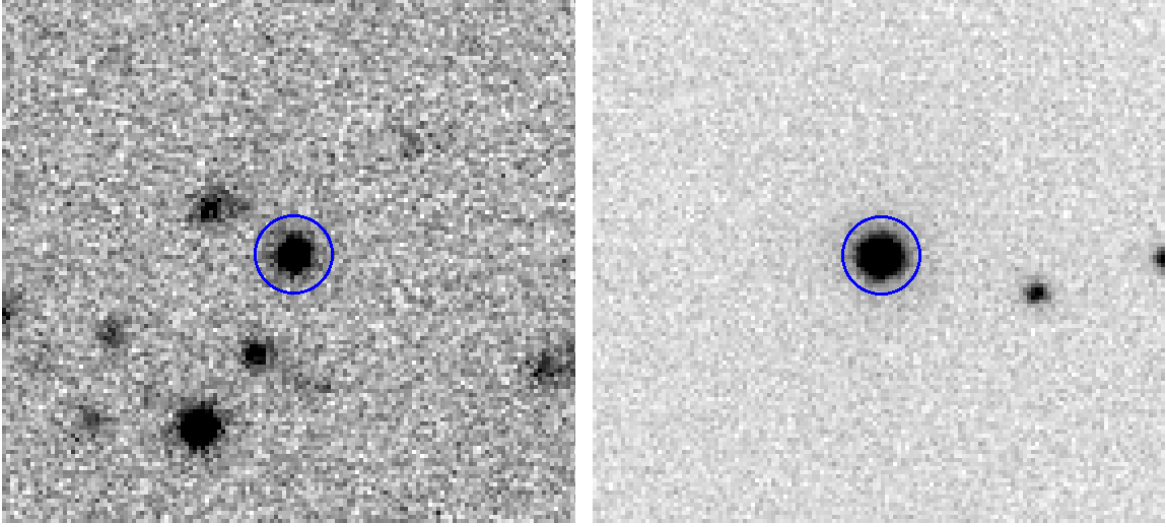
Figure 6. Left: The SN candidate OGLE-2014-SN-094 observed on 2015 Nov. 11. Right: The SN II in SN 2015J at z \sim 0.0054 observed on 2015 Sept. 15. The blue annuli represent the position identified by our pipelines
