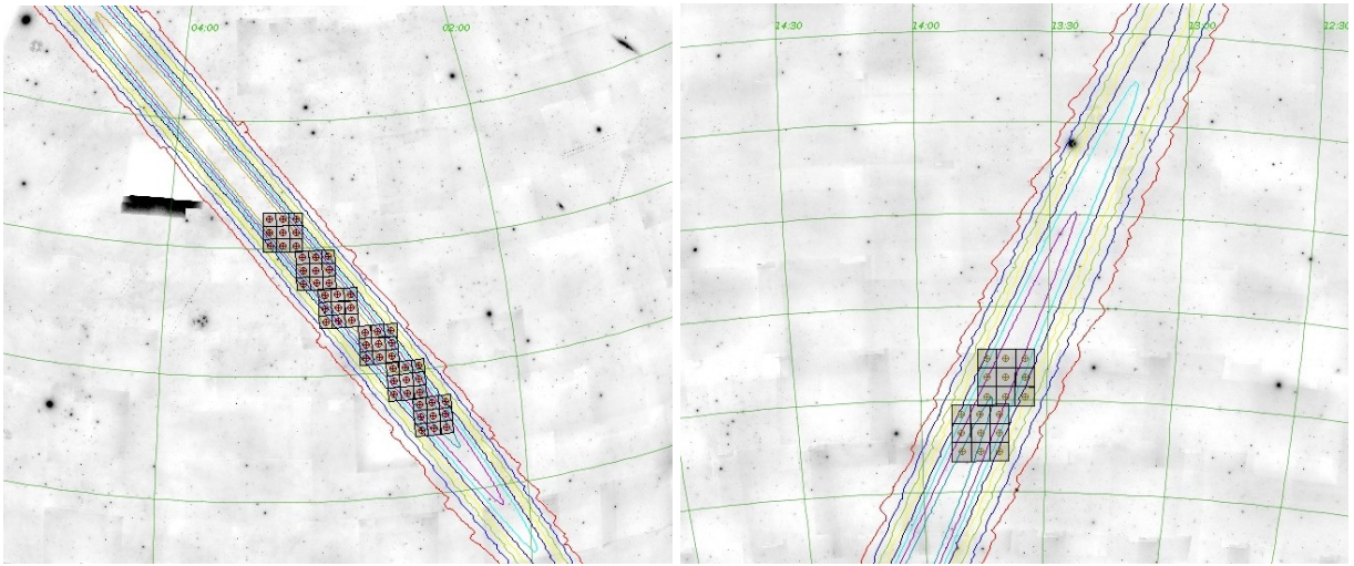
Figure 2. Footprints of the VST r band observations over the contours of the initially distributed BAYESTAR localization map of GW151226. From left to right, the VST coverage in the northern and southern hemispheres is shown. Each square represents the VST Observing Block of 3 \times 3 \text{ deg}^2 . The lines represent the enclosed probabilities from a 90% confidence level to a 10% confidence level in steps of 10%. The eight tiles enclose a localization probability of \sim 9\% . DSS-red image is shown in the background. An interactive skymap can be found in https://www.grawita.inaf.it/highlights/ .
