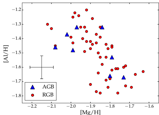
Figure 5. Same as Figure 4, but for Mg and Al.
