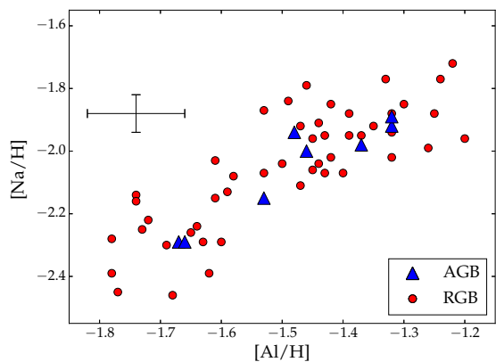
Figure 6. Same as Figure 4, but for Na and Al.
