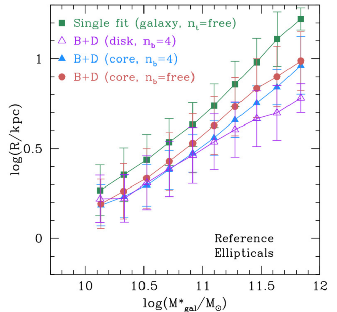
Figure B2. Same as Fig. B1, with equivalent symbols, but for the reference elliptical sample.
