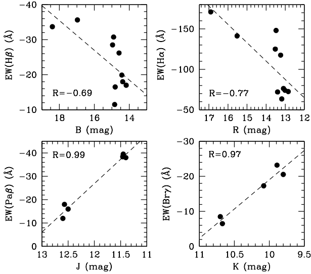
Fig. 5. Equivalent width of optical ( upper panels ) and near-IR ( lower panels ) H I recombination lines as a function of the underlying continuum (in magnitudes). In each panel, the linear fit through the data is shown with a dashed line, and the correspondent regression coefficient is indicated.
