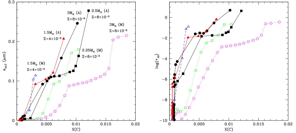
Figure 2. The variation of the size of the olivine (oxygen-rich phases) and solid carbon (carbon stars) dust grains (left-hand panel) and of the optical depth at 10\ \mu\text{m} (right) in the same models shown in Fig. 1. On the abscissa, we show the surface carbon abundance, increasing during the AGB phase. Symbols along the tracks in the left-hand panel indicate the initial mass and whether the MONASH (M) or ATON (A) code was used for the calculation.
