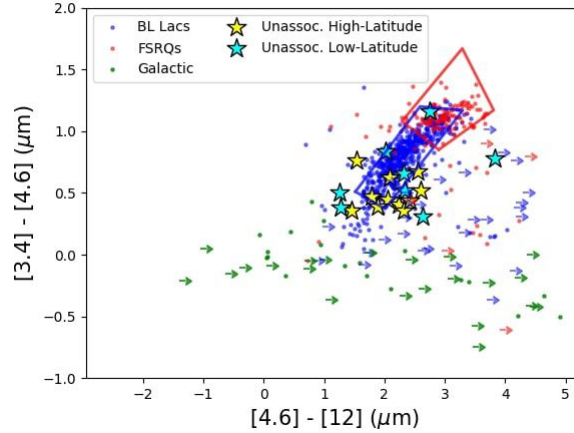
Figure 3. The WISE blazar strip in the color space w_1 ( 3.4\mu\text{m} ) – w_2 ( 4.6\mu\text{m} ) vs w_2 - w_3 ( 12\mu\text{m} ). The blue and red circles represent 439 known BL Lacs and FSRQs used in our machine learning algorithm while known Galactic sources are in green. The coordinates for the strip can be found in Massaro et al. (2012) . The arrows represent sources with only an upper limit on the w_3 magnitude. Two Galactic sources with a w_1 - w_2 value < -1 are not shown to improve readability.
