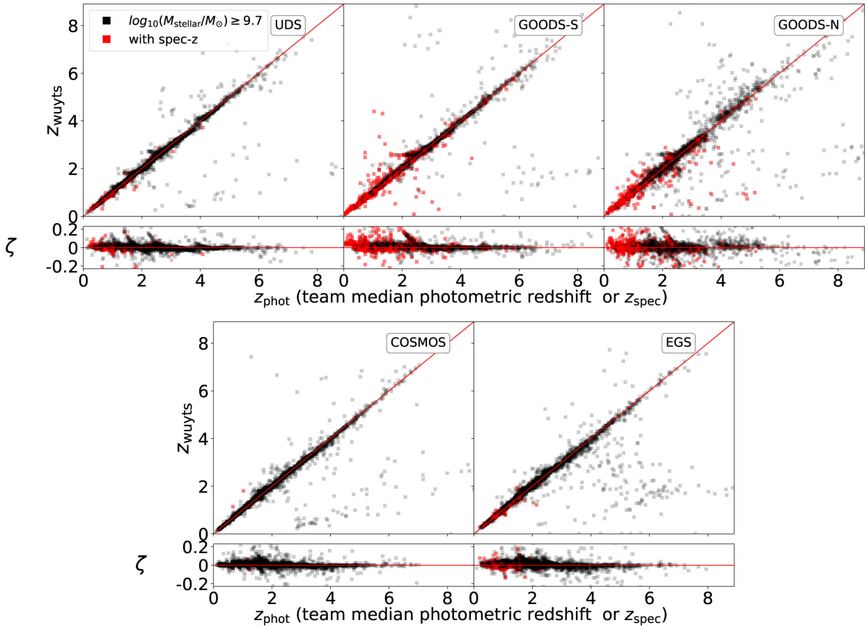
Figure A1. Comparison between the single participant (S. Wuyts) P(z) -based redshifts ( z_{\text{wuyts}} ) to the CANDELS team z_{\text{phot}} values for \log_{10} M_{\text{stellar}}/M_{\odot} \geq 9.7 galaxies (black squares) and those with spectroscopic redshifts (red squares) for five CANDELS fields. In each panel, the top portion of the figure compares both redshift estimates with one-to-one correspondence (red line), and the bottom portion visualizes the redshift normalized scatter defined as \zeta = (z_{\text{wuyts}} - z_{\text{phot}})/(1 + z_{\text{phot}}) centred on zero. We find that the S. Wuyts redshift estimates best match to the CANDELS team values with a median outlier fraction of 1.5 per cent and 3 per cent for z_{\text{phot}} and z_{\text{spec}} samples, respectively (see the text in Appendix for details).
