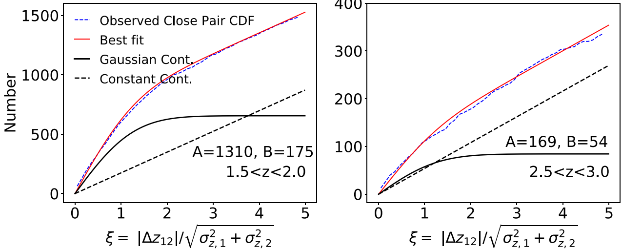
Figure 13. The CDFs of \xi = |\Delta z_{12}|/\sqrt{\sigma_{z,1}^2 + \sigma_{z,2}^2} (from equation 1) for projected pairs satisfying our fiducial 5 \text{ kpc} \leq R_{\text{proj}} \leq 50 \text{ kpc} selection (blue dashed, narrow line) as described in Section 5.3.1 for two redshift bins: 1.5 < z < 2 (left) and 2.5 < z < 3 (right). In each redshift-bin panel, following the equation N(\xi \leq c) = A/\sqrt{2\pi} \int_0^c \exp^{-x^2/2} dx + Bc , the best-fitting curve to the CDF is shown in narrow solid-red line. The breakdown of the best-fitting curve into Gaussian and background contributions are shown in bold solid-black and bold-dashed lines, respectively, and we print the best-fitting values ( A and B ) in each panel.
