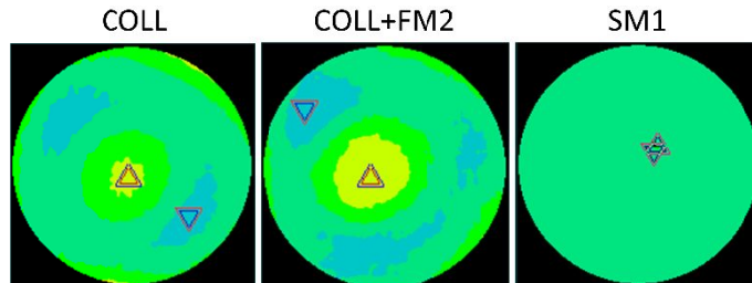
Figure 5. Wavefronts (obtained by the average of 100) of the main optical elements used during M2 alignment, the collimator, the large 45°-oriented flat mirror and the spherical gauge.
