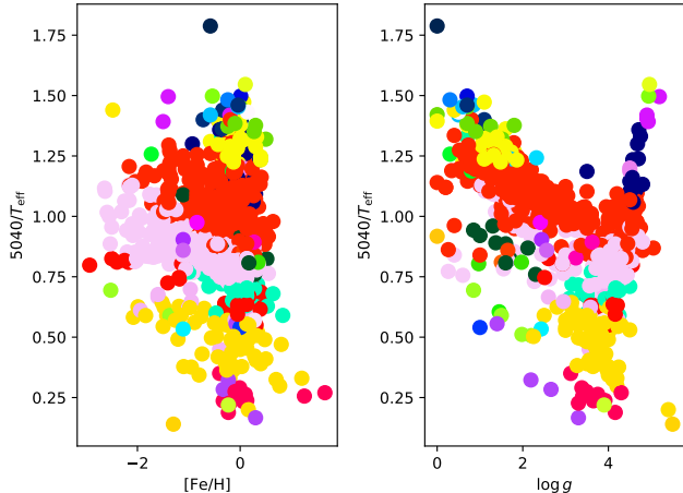
Figure 4. Effective temperature T_{\text{eff}} , metallicity [\text{Fe}/\text{H}] , and surface gravity g of the stars in the MILES stellar library (Falc3n-Barroso et al. 2011). Each datum is assigned a color based on its assigned cluster from the hierarchical-clustering algorithm (Section 5). Some clusters contain a single star, whereas others include about a hundred stars. Cluster boundaries generally do not follow lines of constant stellar parameter due to the degeneracy between the three physical parameters.
