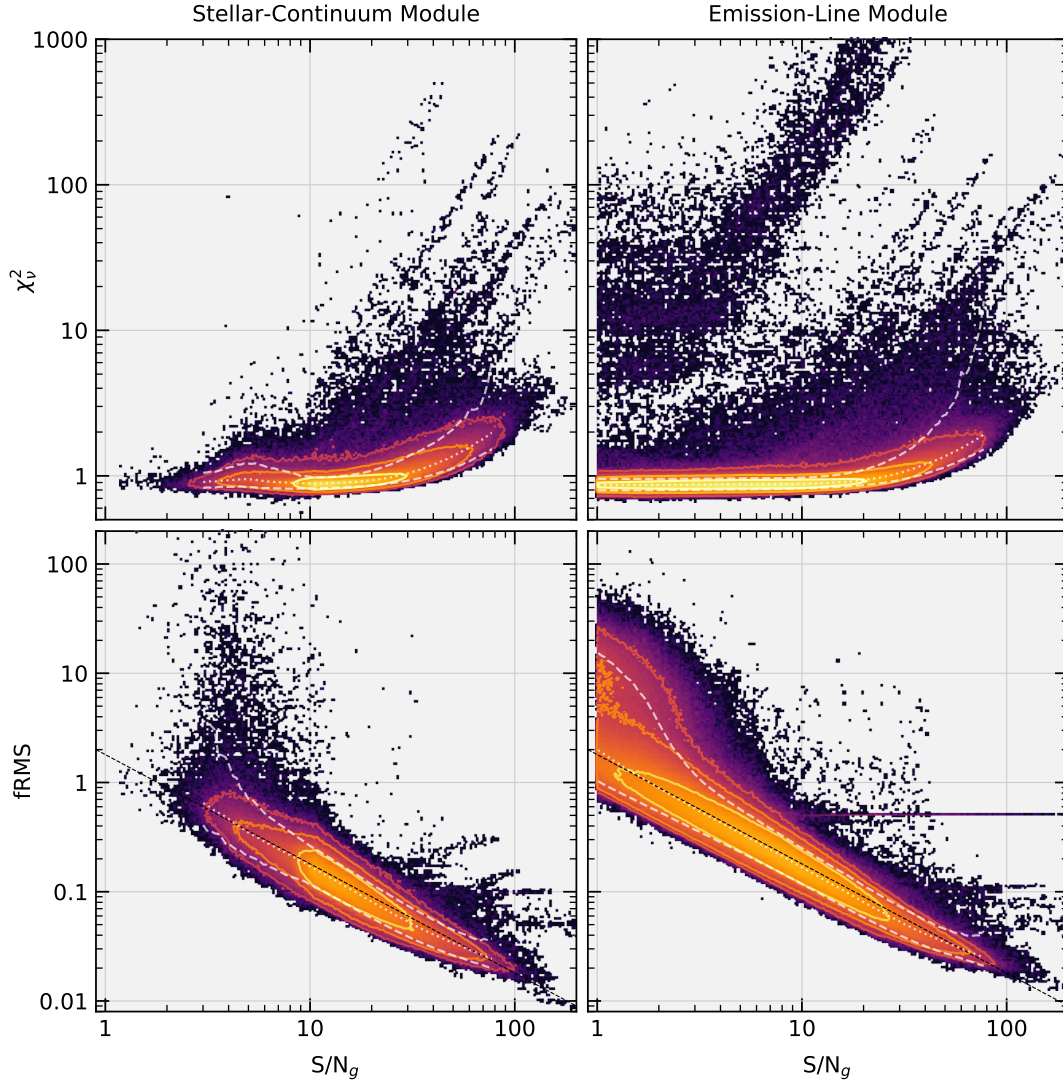
Figure 27. The distribution of \chi_\nu^2 (top) and fRMS (bottom) as a function of S/N_g for all spectra fit in DR15 using the HYB10-GAU-MILES HC approach, excluding datacubes marked as CRITICAL by the DRP or results masked by the relevant DAP module. The difference in the S/N_g distributions for the results of the stellar-continuum module (left) and the emission-line module (right) are because, for the hybrid approach, the stellar-continuum module analyzes the Voronoi-binned spectra, whereas the emission-line module uses the individual spaxels. Note that the S/N_g distribution in the left panels show there are quite a few binned spectra that do not meet the S/N_g \gtrsim 10 threshold. The density of spectra at each location is indicated by the color, where density increases from darker to lighter colors. The three colored contours in each panel enclose 68%, 95%, and 99% of the fitted spectra. That is, populated regions outside the largest contour represent 1% of all MaNGA spectra fit in DR15. The dotted and dashed white lines show, respectively, the 1%, the median and 95% interval at fixed S/N_g .
