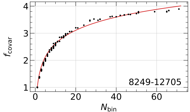
Figure 10. The computed factor that properly rescales noise vectors computed without accounting for covariance to those that do, f_{\text{covar}} , as a function of the number of binned spaxels, N_{\text{bin}} , for the Voronoi bins constructed for observation 8249-12705 (points). These data are based on the median ratio obtained from the direct calculation of the covariance matrix in 11 wavelength channels spanning the full spectral range of the data. For comparison, the nominal calibration, f_{\text{covar}} = 1 + 1.62 \log(N_{\text{bin}}) , from Law et al. (2016) is shown in red.
