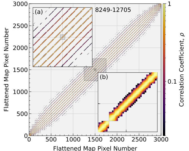
Figure 7. The correlation matrix in channel 1132 ( \lambda = 4700\text{\AA} ) of datacube 8249-12705 for all spaxels with S/N_g > 1 . The correlation matrix is symmetric and has a correlation coefficient of \rho = 1 along the matrix diagonal, by definition. The majority of the matrix is empty with \rho = 0 . The inset panels provide an expanded view of two matrix subregions: Panel (a) shows \pm 250 pixels around the matrix center as indicated by the large gray box, and panel (b) shows \pm 20 pixels around the matrix center as indicated by the small gray box, also shown in panel (a). The diagonal banding in panel (a) is an artifact of the ordering of adjacent pixels in the flattened vector of the datacube spatial coordinates; adjacent pixels are separated by the width of the map in one on-sky dimension. The number of bands in panel (a) roughly matches the width in pixels along the main diagonal with non-zero \rho in panel (b) as expected by the spatial correlation acting along both on-sky dimensions.
