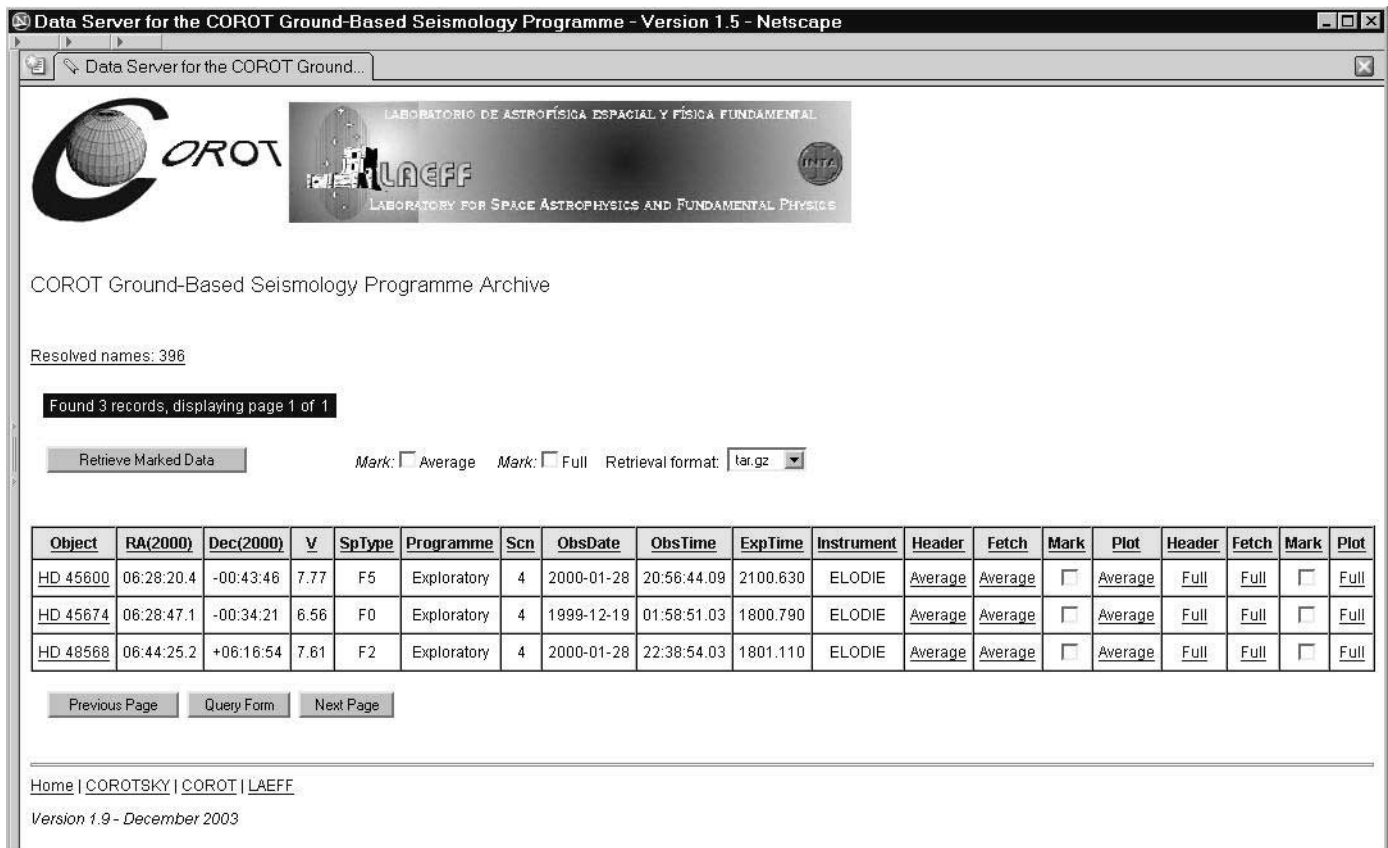
Fig. 2.—Result of the search displayed in Fig. 1. For this example, the spectroscopic output field in HTML format was chosen.
