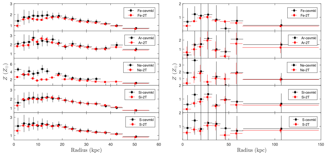
Figure 6. The abundance profiles of Fe, Ar, Ne, Si, and S for the Centaurus (left-hand panels) and Abell 1991 (right-hand panels) obtained with the cevkm1 model (filled black squares) and our reference two-temperature vapEc modelization (filled red squares). The points of the cevkm1 model have been slightly shifted along the x -axis for clarity.
