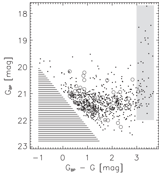
Figure 5. Top: G_{BP} versus G_{BP} - G for all objects. The hashed area is where objects are missed due to the G -band magnitude limit. Open circles are objects with SDSS counterparts. The grey shaded area shows where we expect the G_{BP} - G colour of these objects to occupy.
