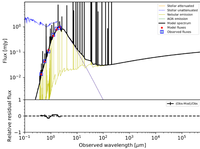
Figure 9. The best SED fit to the NGC 6384 NSC using six-band optical-NIR photometry ( HST : F450W , F606W , F814W , and LBT/LUCI : J , H , K S ). The fluxes are from the model magnitudes in Table 1 obtained via 2D image modelling (in Section 3.2). SED fitting details in Section 3.3.
