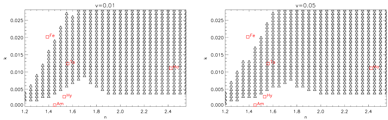
Fig. 11. The plots display with black triangles the regions of the n - k space (real and imaginary parts of refractive index respectively) that satisfy the two constraints 0.85 < \omega_0 < 0.95 and 0.22 < g < 0.52 for any r_{\text{eff}} in the range 0.3 - 3.0 \mu\text{m} . Red squares provide, for reference, the refractive indices at 4.8 \mu\text{m} for different putative components of Jupiter's clouds. Hy : \text{N}_2\text{H}_4 , from Clapp and Miller, Am : \text{NH}_3 , from Howett et al., Fe : \text{NH}_4\text{SH} , from Ferraro et al., Ho : \text{NH}_4\text{SH} , from Howett et al., To : tholin type 2 from Imanaka et al. a. For a size distribution variance of 0.01 b. for a size distribution variance of 0.05.
