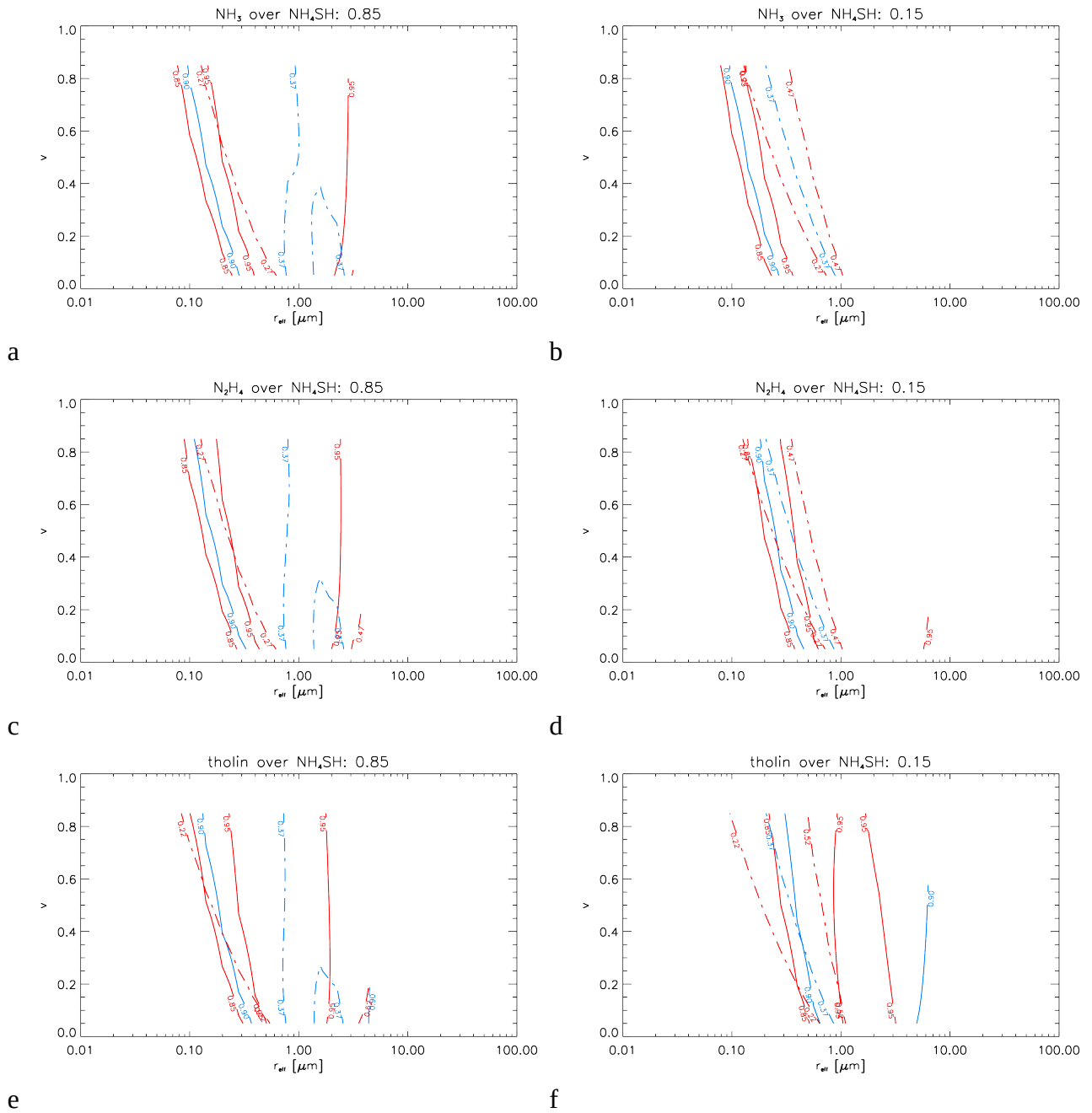
Fig. 12. As fig. 10, for coated particles formed by a \text{NH}_4\text{SH} core (Howett et al.) and different coatings. a.-b. \text{NH}_3 coating. c.-d. \text{N}_2\text{H}_4 coating e.-f. tholin coating. 0.85 and 0.15 labels provide the core-to-particle radii ratio (0.85 large core, 0.15 small core)
