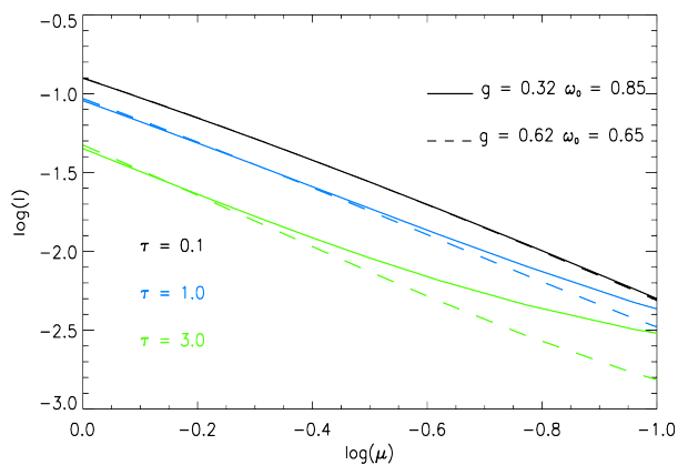
Fig. 2 Examples of theoretical limb darkening functions for typical Hot-Spot conditions, for different cloud opacities \tau . \mu is the cosine of emission angle \epsilon . Note that both axes are in logarithmic form, to highlight deviations from the Minnaret's formulation (see text).
