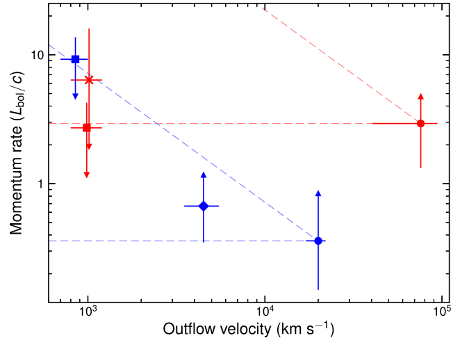
Figure 1. Momentum rate (in units of L_{\text{bol}}/c ) against velocity of the multi-phase outflows in IRAS F11119+3257 (red) and Mrk 231 (blue). The different symbols refer to the outflow type: Fe K (dot), BAL (diamond), OH (cross), and CO (square). The dashed horizontal and diagonal lines correspond to momentum and energy conservation. Error bars ( 1\sigma ) are purely statistical, while arrows indicate whether a given measure should be considered as a lower or an upper limit (see the text for details).
