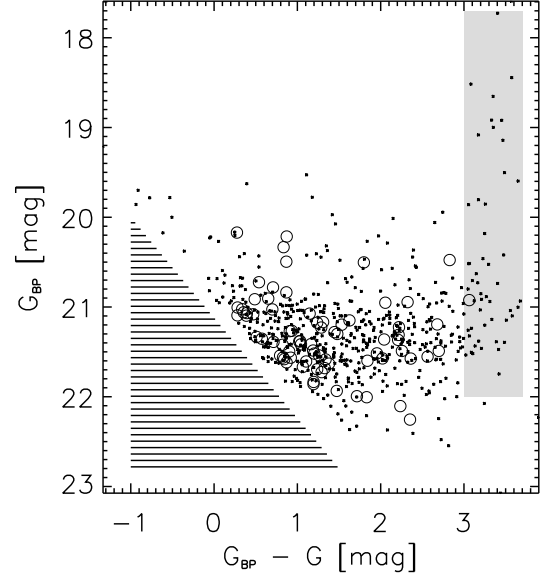
Figure 5. Top: G_{\text{BP}} vs. G_{\text{BP}} - G for all objects. The hashed area is where objects are missed due to the G band magnitude limit. Open circles are objects with SDSS counterparts. The grey shaded area shows where we expect the G_{\text{BP}} - G colour of these objects to occupy.
