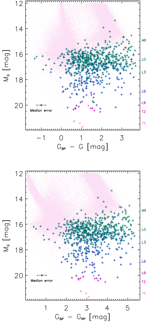
Figure 4. Colour-magnitude diagrams for absolute G vs. G_{\text{BP}} - G (top) and G_{\text{BP}} - G_{\text{RP}} (bottom). The light pink points are all objects within 100 pc, the crosses are the GUCDScat entries colour-coded by spectral type as indicated on the right hand side. Plotted in the lower left are error bars that are equivalent to the median uncertainty.
