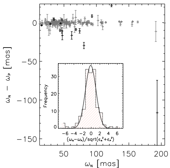
Figure 2. Differences between Gaia DR2 and published parallaxes vs. Gaia DR2 parallaxes. Error bars are combined Gaia DR2 and published uncertainties plotted in grey. The large outlier is J1506+7027 discussed in the text. In black, all object with parallaxes differing by more than 2.5 times the combined uncertainties (listed in Table 4). The insert is a plot of the distribution of the ratio of parallax differences to combined uncertainties as shown in Equation 1
