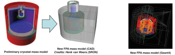
Preliminary cryostat mass model New FPA mass model (CAD) Credits: Henk van Weers (SRON)
