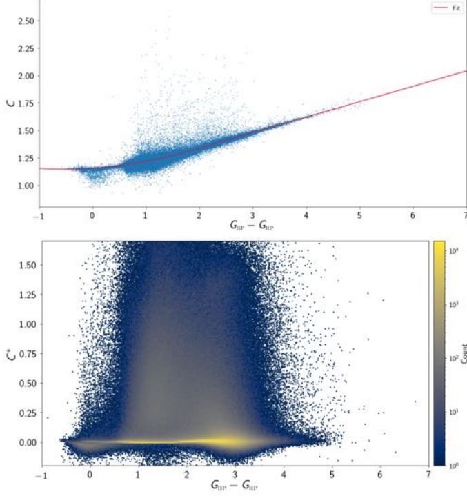
Fig. 18. Determination of the BP and RP flux excess dependence on G_{BP} - G_{RP} colour and its application to define the corrected excess factor C^* . Top panel: BP and RP flux excess vs. G_{BP} - G_{RP} colour for the set of standard sources from Stetson (2000) secondary standards and Ivezić et al. (2007) . The red line represents the combined fit based on two different polynomials for the bluer-end and the central region and a linear fit for the red-end. Bottom panel: corrected flux excess factor C^* vs. G_{BP} - G_{RP} colour for a set of nearby sources selected from the Gaia EDR3 archive.
