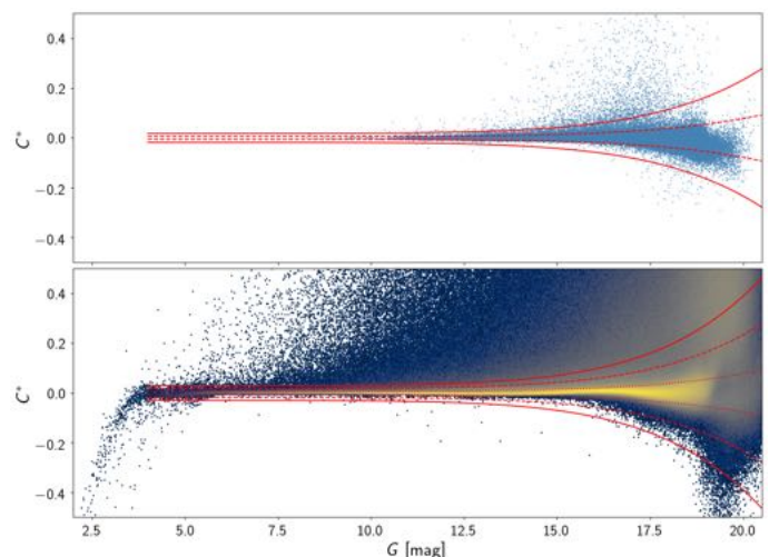
Fig. 31. Corrected BP and RP flux excess vs. magnitude for the Stetson and Ivezić dataset (top panel) including the \pm\sigma (solid) and \pm3\sigma (dashed) scatter lines and for the nearby source dataset (bottom panel) including the \pm\sigma (solid), \pm3\sigma (dashed) and \pm5\sigma (dotted) scatter lines. The scatter lines are defined by Eq. 18 with the fit coefficients provided in the text.
