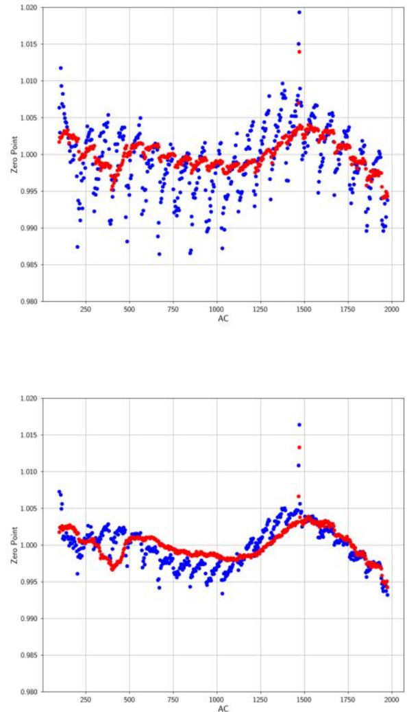
Fig. G.1. CCD response as a function of AC position as derived from the SS calibration. The top panel shows the response when the flux loss has been modelled and corrected only in the range \pm 2 pix; the bottom panel shows the response when the flux loss has been modelled and corrected in the range \pm 4 pix. The blue dots show the preceding FoV; the red dots show the following FoV.
