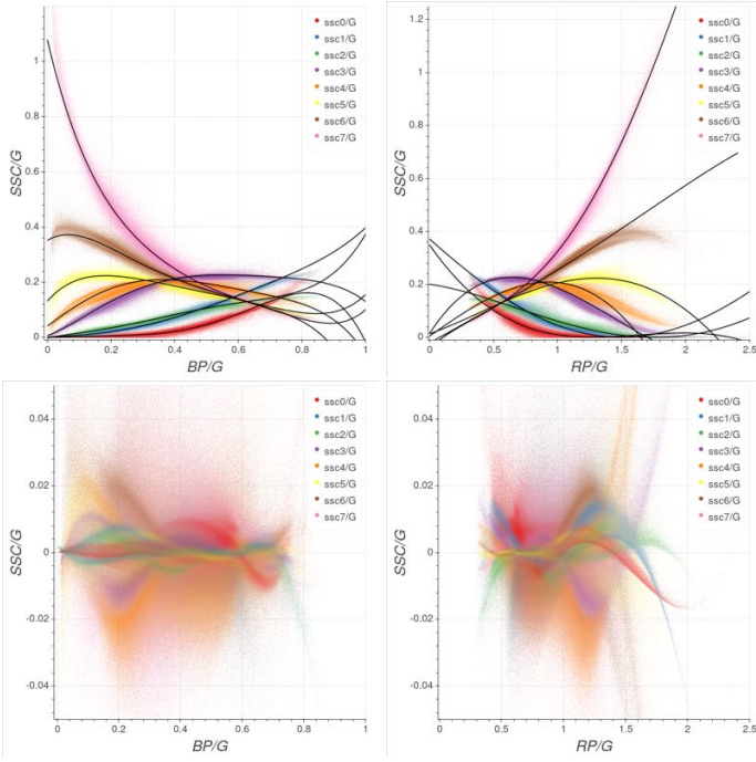
Fig. E.1. Results of the estimation procedure. Top: Distribution of sources in the SSC/G vs. XP/G space (colour-coded according to the legend) and the results of the corresponding fits (black lines). Bottom: Residuals.
