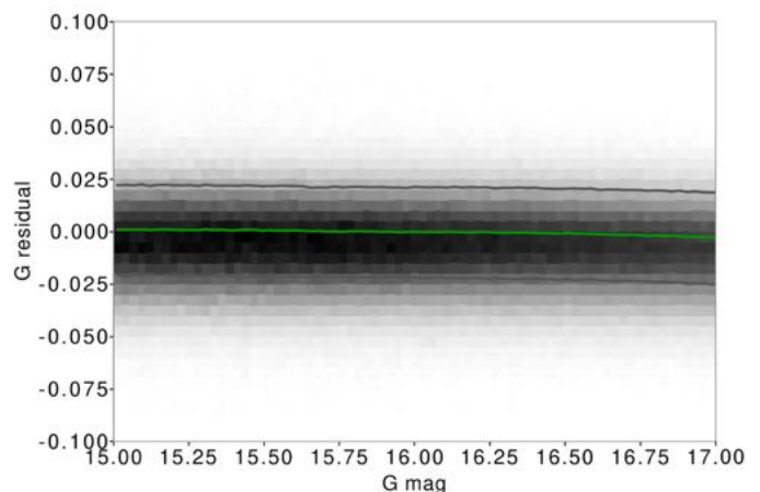
Fig. 17. Comparisons of Gaia EDR3 with APASS (upper plot) and SDSS DR15 (lower plot) showing that no discontinuities are detected at G = 13 or G = 16 .
