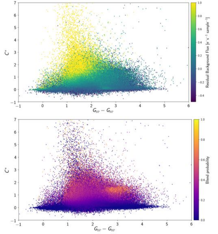
Fig. 19. Effect of residual background flux and blending probability on the corrected BP and RP flux excess. Top panel: Distribution of corrected BP and RP flux excess vs. G_{BP} - G_{RP} colour for a subset of nearby sources fainter than 17 in G -band. The symbols are colour coded by the source median residual background as measured from the BP spectra. Bottom panel: Distribution of corrected BP and RP flux excess vs. G_{BP} - G_{RP} colour for the same sources shown in the top panel but colour-coded by blend probability (see text for details). For these plots sources have been further selected to retain sources where the blend probability for BP and RP was in agreement to within 50%.
