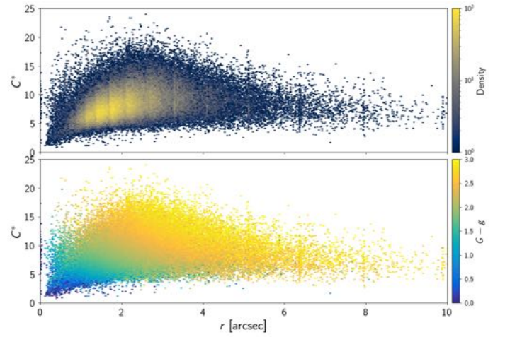
Fig. F.1. Dependence of the corrected BP and RP flux excess factor C^* with the apparent size of the galaxy provided in terms of its de Vaucouleurs radius for a sample of \approx 146 thousand galaxies selected from SDSS DR12. The top panel shows the density, the bottom panel the colour scale shows the difference between the Gaia G -band magnitude and the SDSS g magnitude.
