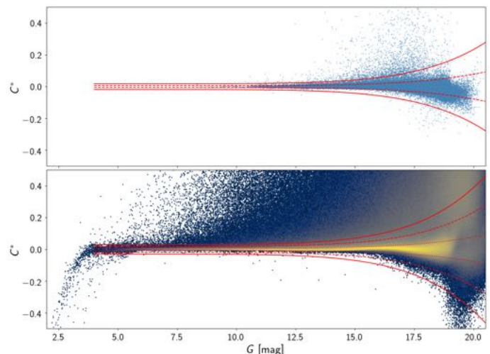
Fig. 31. Corrected BP and RP flux excess vs. magnitude for the Stetson and Ivezić dataset (top panel) including the \pm\sigma (solid) and \pm3\sigma (dashed) scatter lines and for the nearby source dataset (bottom panel) including the \pm\sigma (solid), \pm3\sigma (dashed) and \pm5\sigma (dotted) scatter lines. The scatter lines are defined by Eq. 18 with the fit coefficients provided in the text.
