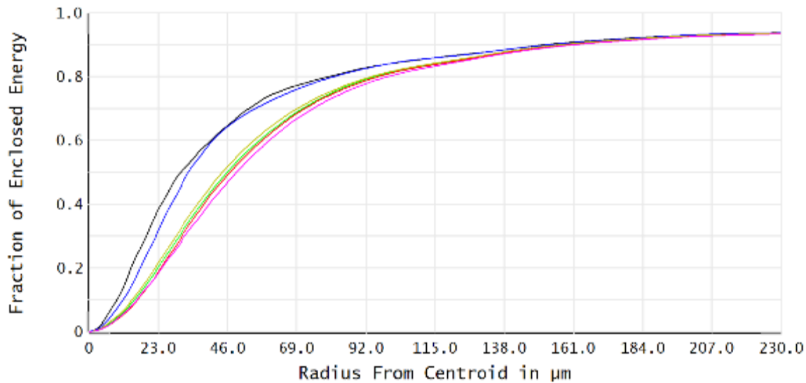
Figure 8 Encircle energy for PSF f/34 (IFU100) case.
