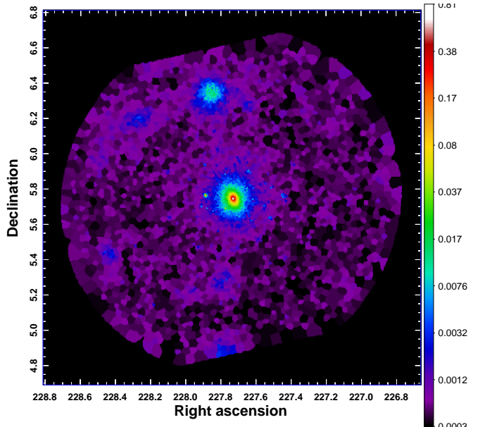
Figure 4. ROSAT /PSPC surface-brightness image of A2029 obtained using Voronoi tessellation (Cappellari & Copin 2003), in units of \text{cts s}^{-1} \text{ arcmin}^{-2} . Each Voronoi bin includes an average of 20 counts.
