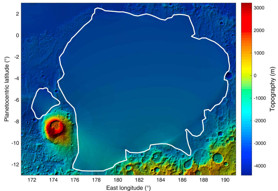
Figure 5. Topographic map of the Lucus Planum area, based on the MOLA data set. The white contours identify the areas in which MOLA topography was removed, and then the base of the Lucus Planum and Apollinaris Patera deposits was interpolated from the remaining topographic information through the natural neighbor method.
