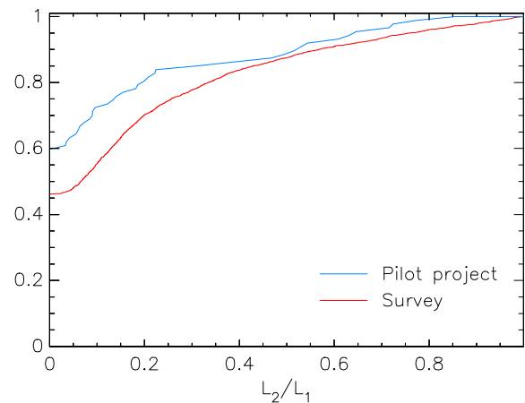
Figure 16. Cumulative distribution of the ratio of flux densities L_{2, \text{ref}}/L_{1, \text{ref}} for targets from the pilot project (blue line) and the survey (red line). Sometimes the fitting procedure re-arranges the order of the components, in which case the component labeled ‘2’ becomes the brightest polarized component. In those cases we swap L_{1, \text{ref}} and L_{2, \text{ref}} , so that the ratio between these two flux densities is again < 1 .
