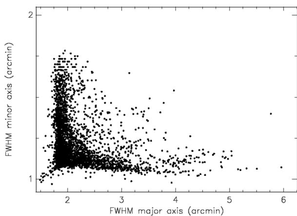
Figure 2. Size of the restoring Gaussian beam used to create the final CLEANed image for each ATCA field, at 2.2 GHz. Note the difference in scale between the horizontal and vertical axes.
