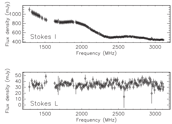
Figure 4. Stokes I and L frequency spectra for the brightest source in Stokes I in the target field of PKS B1923-328 (top and bottom panel, respectively). The bump in the Stokes I spectrum is due to confusion with another source in the field of view, but this bump is missing from the polarization data. Error bars indicate 1\sigma uncertainties. We used standard error propagation to calculate the errors in L , allowing for the measurement uncertainties in Stokes Q and U to be different in each frequency channel.
