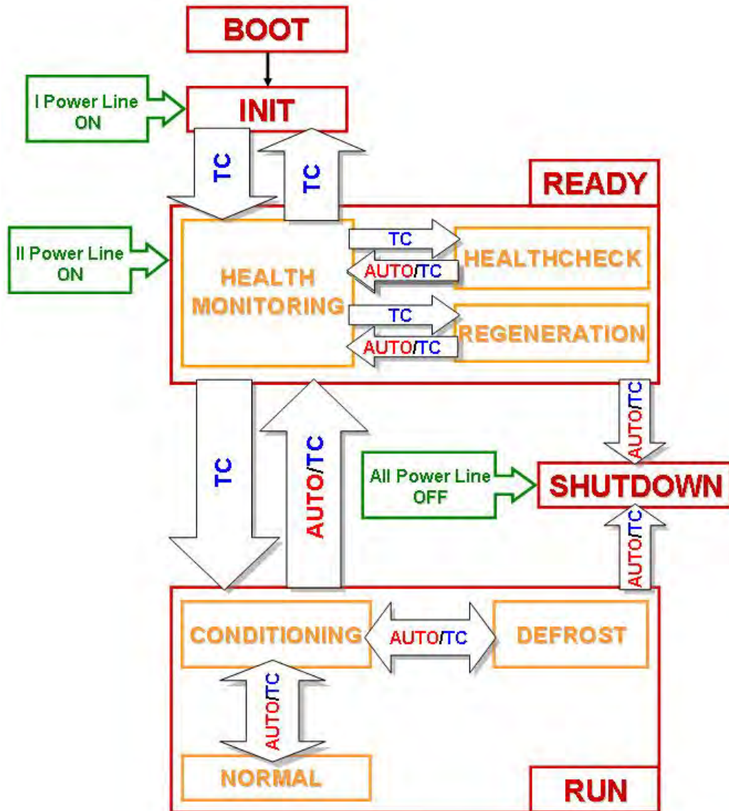
Figure 8-11: Operating Modes
