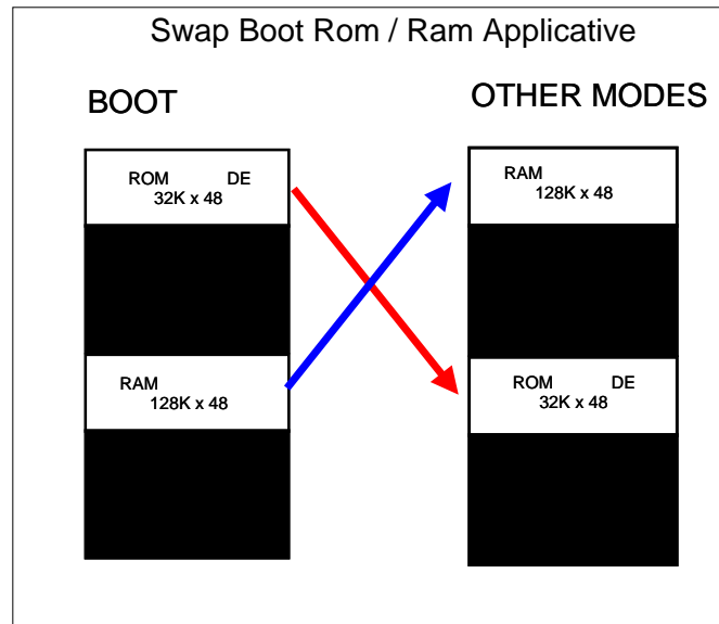
Figure 8-16: Swap PM PROM / PM RAM
