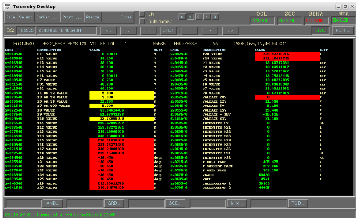
Figure A3-47: The SA013540 AND – Calibrated parameters from housekeeping in ASW modes
