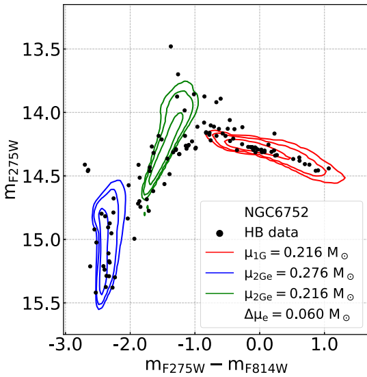
Figure 2. The m_{F275W} - m_{F814W} versus m_{F275W} CMD for NGC 6752 where we overplot our best-fitting simulations as contour plots, with red and blue respectively for the 1G and the 2Ge. The green contour plot represents the 2Ge simulation but with the same mass-loss value of the 1G, as indicated in the label.
