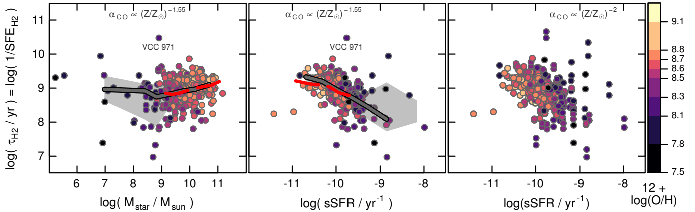
Fig. 11. Logarithm of H 2 depletion time \tau_{\text{H}_2} plotted against M_{\text{star}} in the left panel , and against specific SFR in the middle and right panels . In the middle and right panels , the heavy dark-gray curves correspond to the binned data medians; only bins with 5 or more galaxies are shown. The gray shadowed regions indicate the range of \pm 1\sigma of the binned data. The heavy red long-dashed curves give the xCOLDGASS medians (Saintonge et al. 2017). The right panel shows the impact of using \alpha_{\text{CO}} \propto (Z/Z_{\odot})^2 , rather than the value we find here. Galaxies are colored with 12 + \log(\text{O}/\text{H}) is as in Fig. 2.
