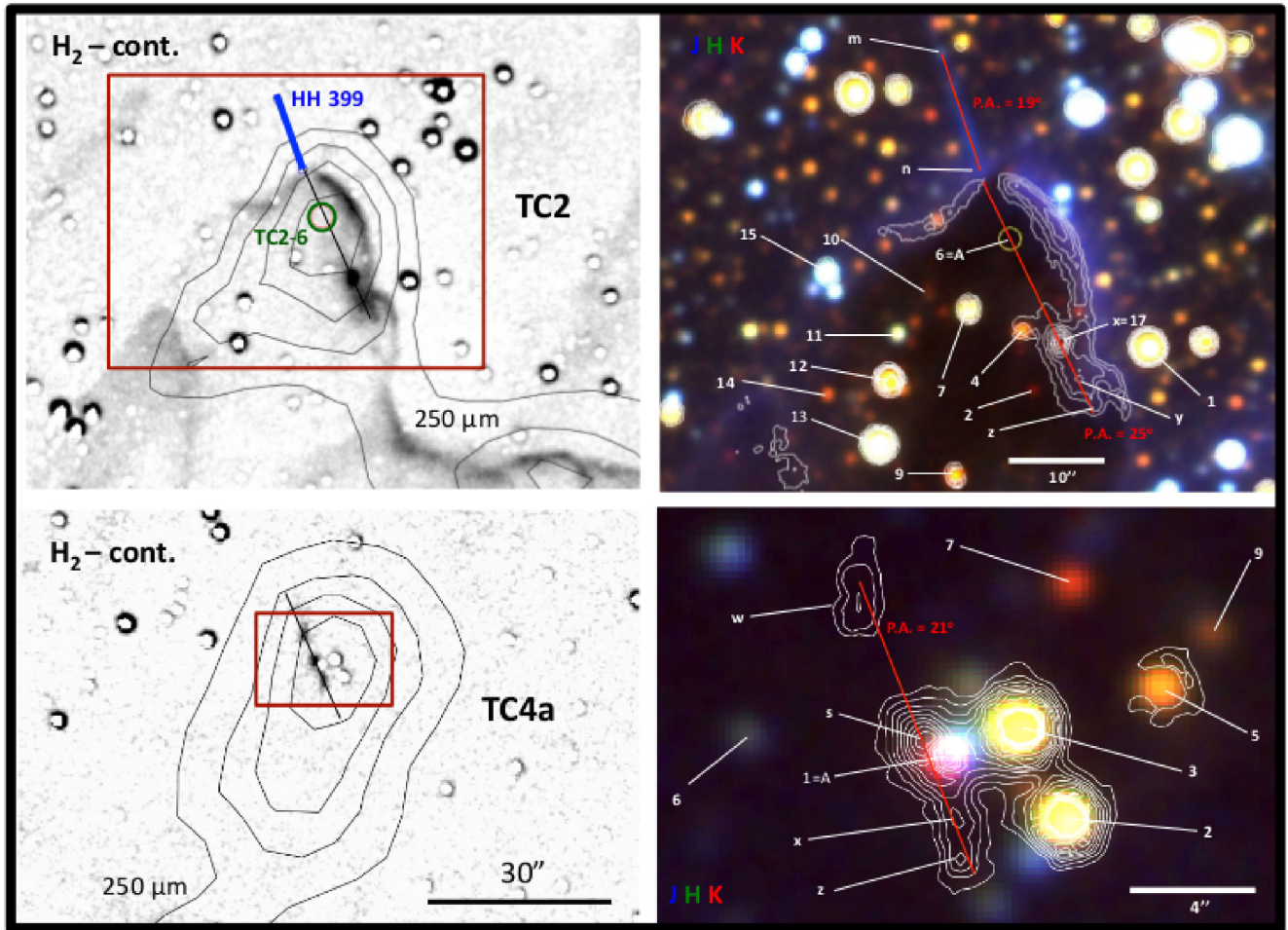
Figure 13. Magnified views of two regions where new shocked molecular hydrogen emission knots are discovered, TC2 and TC4a (upper and lower panels, respectively). On the left, the Herschel 250 μm emission contours are plotted over the continuum-subtracted molecular hydrogen line (2.12 μm) emission images. The straight thin black lines at 23° position angles join the jet and H 2 knots with the putative central driving sources, TC2-6 and TC4a-1. The blue line represents the HH 399 optical and near-IR jet. Panels on the right show close-up sections (marked with dark red rectangles on the left-hand panels) of the JHK s images showing the details of the jets. White contours represent the continuum-subtracted 2.12 μm H 2 emission. The reddest near- and mid-IR sources are labelled with numbers as in Table 4. The letters identify the small H 2 knots and the endpoints of HH 399, all listed in Table 5. Red lines (with corresponding position angles) mark the direction of the proposed flows (see text). The coordinates of TC2-6=A are: \alpha(J2000) = 18^{\text{h}}02^{\text{m}}28^{\text{s}}.6 , \delta(J2000) = -23^{\circ}03'48'' , and those of TC4-1 = A are \alpha(J2000) = 18^{\text{h}}02^{\text{m}}12^{\text{s}}.8 , \delta(J2000) = -23^{\circ}05'47'' . North is at the top, east to the left. Spatial scales are illustrated with horizontal bars
