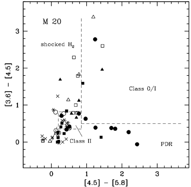
Figure 6. [3.6] - [4.5] versus [4.5] - [5.8] diagram of all sources with IRAC photometry in the studied TCs as listed in Table 4. Broken lines delineate the areas that are occupied by Class 0/I and Class II objects, and also indicated with labels are the approximate zones occupied by shocked \text{H}_2 - and PAHs-dominated emission regions (Ybarra et al. 2014). Symbols are as in Fig. 5.
