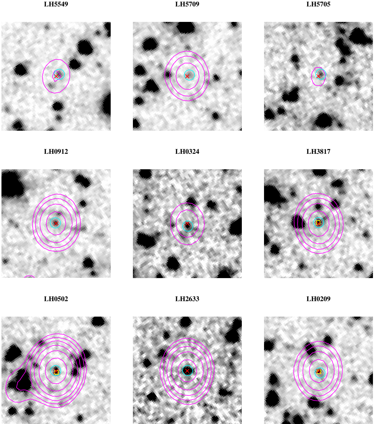
Fig. A.2: Images of the reliable (i.e. reliability >90%) counterparts of IFRSs identified in LH SERVS field. All the images are \sim 40'' \times 40'' wide, North is up and East on the left. The (inverted colours) black-and-white background images are SERVS cutouts, taken from the 3.6 or the 4.5 \mu\text{m} mosaics (depending on which band the reliability has been computed). Superimposed are a red cross (marking the radio peak position, always at the centre of the cutout), a cyan circle (marking the area within which aperture photometry was derived), and a green square (marking the position of the optical counterparts, see Table 5). Also reported are the isophotes of the radio sources (magenta lines, contour levels at 10, 20, 40, 80, 160, 320, 640, and 1280\sigma the radio image noise).
