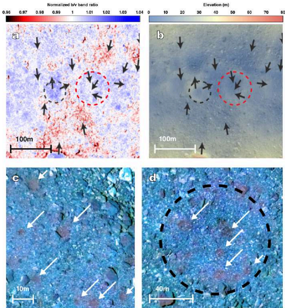
Fig. 4. Examples of crater color. (A) The b/v band ratio map of equatorial craters at 3.05^\circ\text{S} , 128.79^\circ\text{E} (black dashed line) and 1.06^\circ\text{S} , 152.75^\circ\text{E} (red dashed line), which have a higher near-UV index and are considered blue units. (B) An elevation map of the same equatorial craters in (A). These blue units correspond with areas that show recent indications of mass movement away from regionally high elevations, such as from crater rims. Black arrows correspond locations of previously mapped mass movement (43). (C and D) RGB color composites images of small craters (indicated by white arrows), shown on the same color scale as Fig. 1A. As indicated by their color, these craters are consistently redder than Bennu's average terrain, with positive to slightly blue b' to x spectral slopes. The blue crater indicated by the dashed black line in (A), (B), and (D) has been overprinted by several smaller reddish craters.
