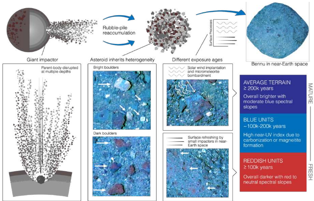
5 Fig 7. Proposed model of color and reflectance diversity. We propose that distinct rock types formed at different depths on Bennu's parent body. After the parent body was catastrophically disrupted by a giant impactor, Bennu accumulated from its debris (4-6) and inherited these distinct materials, leading to the observed heterogeneity among boulders on Bennu. Since Bennu's formation and subsequent transit to near-Earth space, it has been altered by exposure to the space environment, which ultimately results in its moderately blue global color. Small near-Earth impactors also continually refresh the surface, creating craters of comparatively fresh, reddish material, which weather towards bluer colors on a timescale of \sim 10^5 years.
