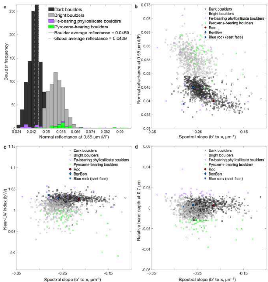
Fig. 2. Variation of boulder color and reflectance on Bennu. (A) Reflectance distribution of boulders (>5 m) on Bennu. The distribution is multi-modal with more than one Gaussian component (31). Shading and colors indicate different classifications of boulders, as indicated in the legend. (B) Normal reflectance versus absolute spectral slope of the same boulder populations; some individual boulders are indicated in the legend. Dark boulders tend to be redder, and their reflectance monotonically decreases with increasing (redder) spectral slopes, whereas bright boulders are bluer and more scattered (31). (C) The near-UV index ( b'/v band ratio) versus the b' to x spectral slope. Dark boulders tend to have a steeper near-UV slope relative to the global average ( >1 ), whereas bright boulders are more often spectrally flat or show a downturn in the near-UV (from the b' to v bands). (D) The relative band depth at 0.7 \mu\text{m} ( w band) versus the b' to x spectral slope. Some boulders show an absorption feature at 0.7 \mu\text{m} (relative w band depth >0 ), indicative of Fe-bearing phyllosilicates. The boulders named Roc ( 23.6^\circ\text{S} , 25.3^\circ\text{E} ; Fig. 3C) and
