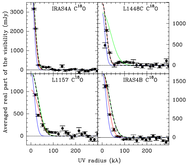
Fig. B.1. C^{18}O uv-plots for IRAS4A (top left), L1448C (top right), L1157 (bottom left) and IRAS4B (bottom right). The data is integrated over \pm 3 \text{ km s}^{-1} around the line centre and radially averaged in bins of 20 m with task uv_circle in MAPPING. Red lines show the result of the circular Gaussian fits to the un-averaged uv data, while the blue and green lines show the results of the elliptical Gaussian fits to the un-averaged uv data along the major and minor axes, respectively. Black dashed lines show the result of the elliptical Gaussian fits with fixed P.A. along the outflow. The parameters of the fits are listed in Table 3.
