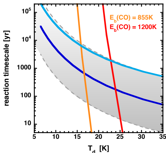
Fig. 7. CO ice depletion timescale (dark blue line) and thermal desorption timescales for binding energies of 855 K (orange line) and 1200 K (red line) as function of the dust temperature for the density profiles of IRAS4B. The light blue line shows the free-fall time for an enclosed mass of 0.5 M_{\odot} . The points of intersection at \sim 17 K and \sim 24 K mark the locations of the CO snow line for the two different values of the binding energy. The grey area shows the range of depletion timescales if the dust density is varied by a factor of ten. For a binding energy of 855 K, the variation of the density translates into a variation of the snow line location at \sim 16 K or \sim 17 K, while for a binding energy of 1200 K, the modified snow line locations would be at \sim 23 K or \sim 25 K.
