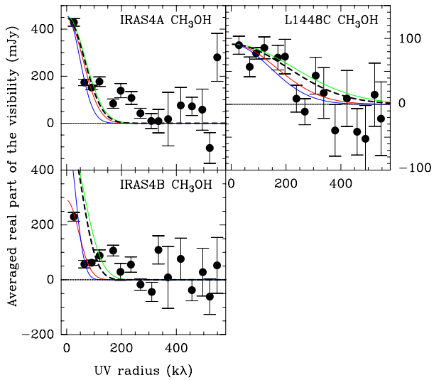
Fig. B.2. Same as Figure B.1, but for CH_3OH in IRAS4A (top left), L1448C (top right), and IRAS4B (bottom left). The data is radially averaged in bins of 50 m with task uv_circle in MAPPING. The parameters of the fits are listed in Table 4.
