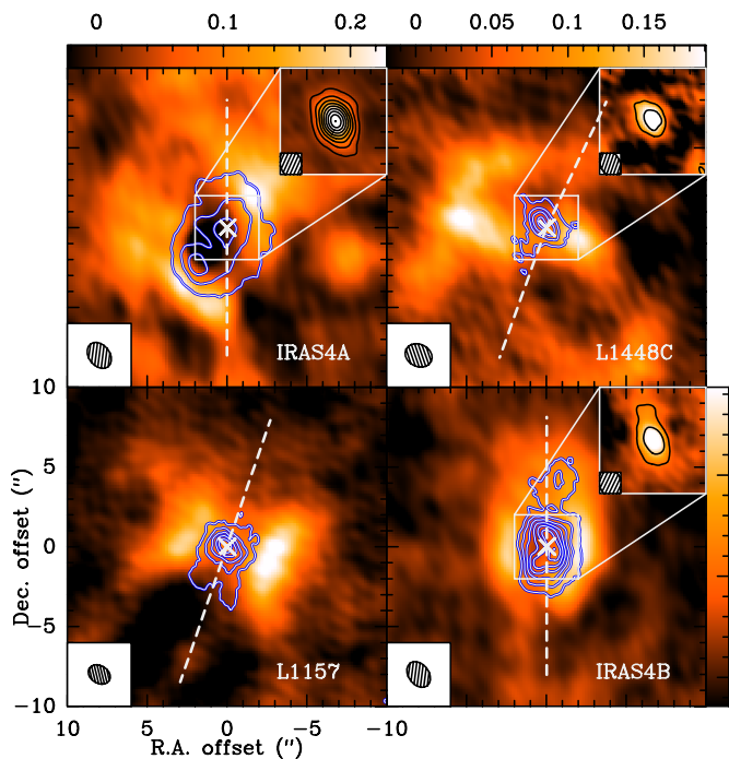
Fig. 1. Anticorrelation between \text{N}_2\text{H}^+ and \text{C}^{18}\text{O} . Colour background: \text{N}_2\text{H}^+ (1–0) emission integrated over all seven hyperfine components. The noise in these maps is \sigma=(0.030, 0.027, 0.025, 0.029) \text{Jy beam}^{-1} \text{ km s}^{-1} for IRAS4A, L1448C, L1157, and IRAS4B, respectively. The wedges show the \text{N}_2\text{H}^+ intensity scale in \text{Jy beam}^{-1} \text{ km s}^{-1} . For the two lower panels the scaling is the same. Contours show emission of \text{C}^{18}\text{O} (2–1) in steps of 6\sigma (IRAS4A and 4B) or 3\sigma (L1448C and L1157), starting at 3\sigma , with \sigma=(0.044, 0.029, 0.031, 0.033) \text{Jy beam}^{-1} \text{ km s}^{-1} for IRAS4A, L1448C, L1157, and IRAS4B, respectively. The inlays in the upper right corners show the methanol emission as colour background and contours in steps of 3\sigma , starting at 3\sigma inside the central 2'' , with \sigma=(0.028, 0.019, 0.027) \text{Jy beam}^{-1} \text{ km s}^{-1} for IRAS4A, L1448C, and IRAS4B. In L1157, the methanol line has not been detected at a 3\sigma level. The filled ellipses in the lower left corner of the panels indicate the synthesized beam sizes of the \text{N}_2\text{H}^+ observations at 3 mm. The dashed white lines illustrate the small-scale outflow directions (see Table 3 and Section 3.1) and the white crosses show the positions of the sources as listed in Table 1.
