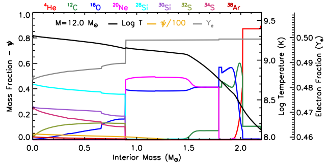
Figure 34. Selected chemical and physical properties (see the legend) of the 9.22 M_{\odot} (left panel) and 12.0 M_{\odot} models when the ONe burning front has reached the center.
