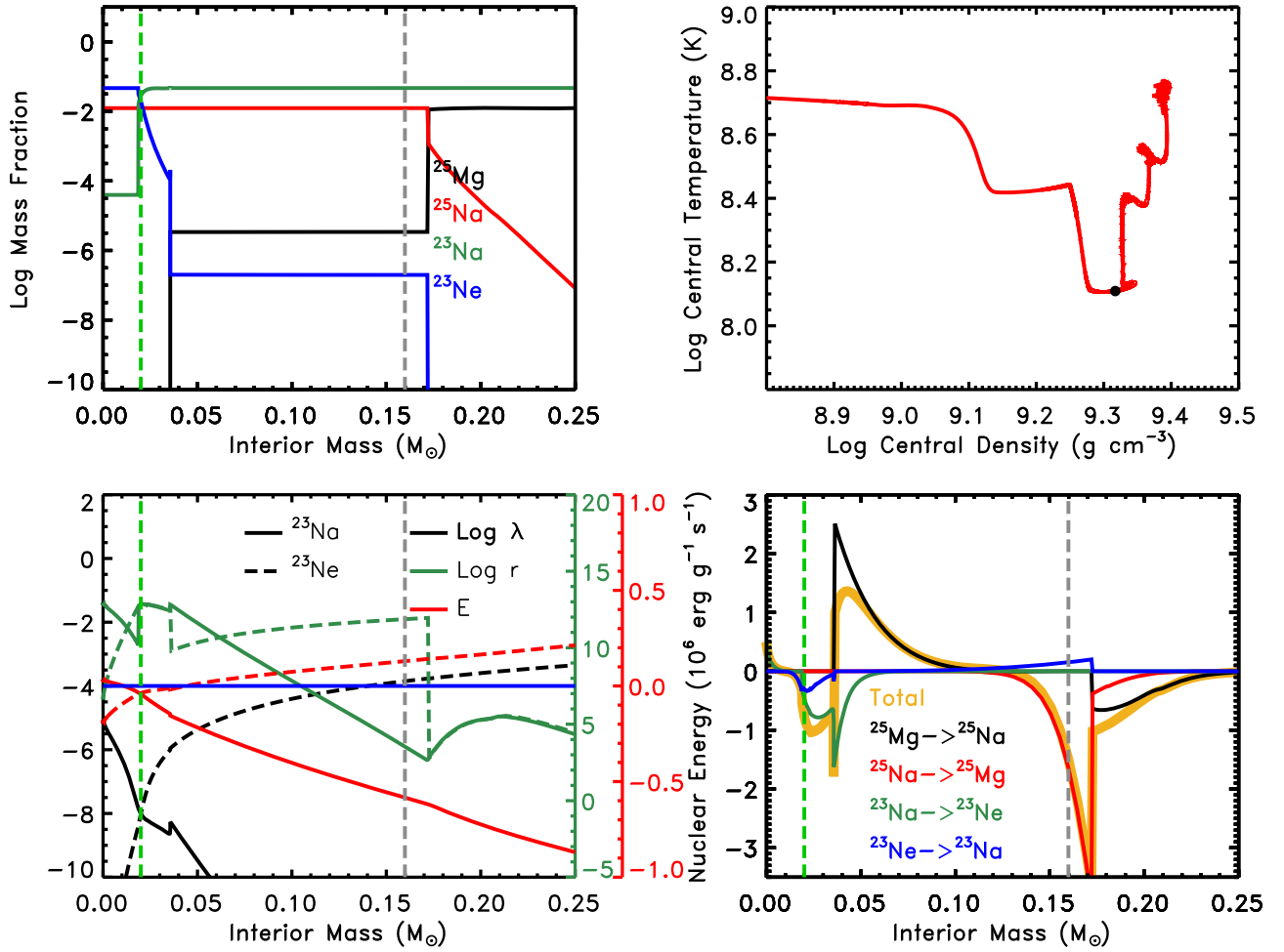
Figure 21. Same as Figure 20 but during a phase in which a convective core, driven by the ^{23}(\text{Na, Ne}) URCA pair, and a convective shell, induced by the ^{25}(\text{Mg, Na}) URCA pair, are formed. The gray and green vertical dashed lines mark the ^{25}(\text{Mg, Na}) and ^{23}(\text{Na, Ne}) URCA shells, respectively.
