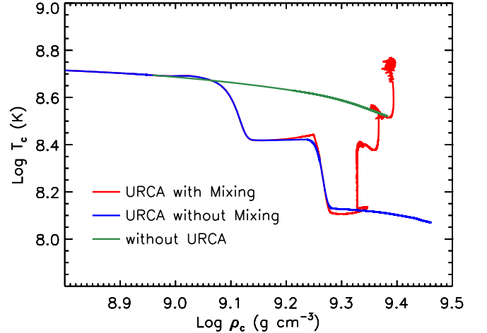
Figure 26. Evolution of the central temperature as a function of the central density for three models of initial mass 9.20 M_{\odot} prior to the onset of the TIR (see text), computed with the following assumptions: URCA processes and convective mixing taken into account (reference model; red line), URCA processes taken into account and convective mixing artificially suppressed (blue line), and URCA processes neglected (green line).
