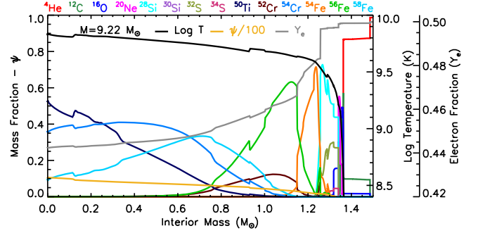
Figure 38. Selected chemical and physical properties (see the legend) of the 9.22 M_{\odot} star at the presupernova stage.
