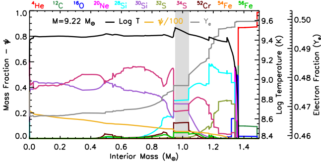
Figure 35. Selected chemical and physical properties (see the legend) of the 9.22 M_{\odot} star at off-center Si-S ignition.
