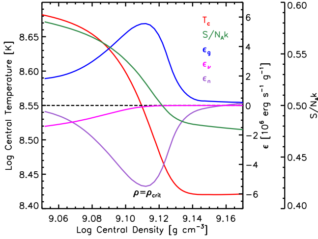
Figure 18. Selected central quantities as a function of the central density of the 9.2 M_{\odot} model during the activation of the ^{25}(\text{Mg}, \text{Na}) pair: temperature (red line, left y-axis), adimensional entropy per baryon (green line, right y-axis), and nuclear (purple), gravitational (blue), and neutrino (magenta) energies (right y-axis).
