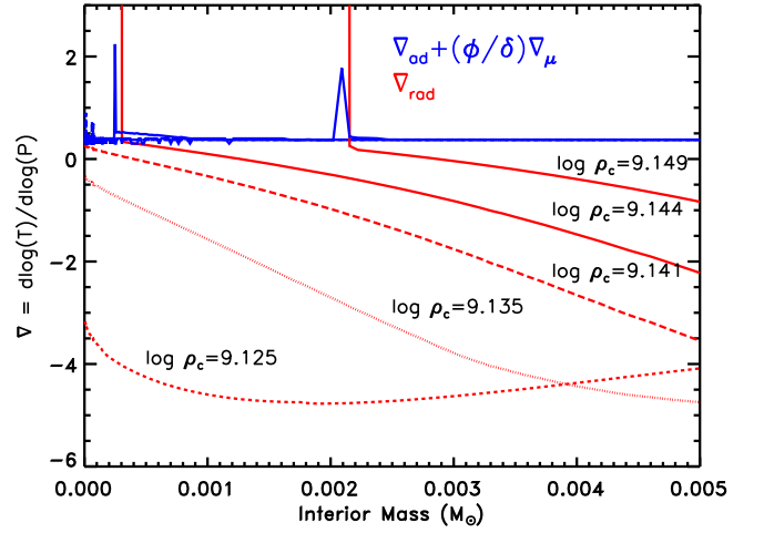
Figure 19. Temperature gradients (see the legend) as a function of the interior mass of the 9.2 M_{\odot} star at selected times during the formation of the convective core associated with the ^{25}(\text{Mg}, \text{Na}) URCA pair, marked by the values of the central densities in units of \text{g cm}^{-3} . According to the adopted stability criterion (see text), convection sets in when the radiative gradient becomes larger than the adiabatic one. Let us remember that the actual temperature gradient used is the adiabatic one in the convective zones and the radiative one in the radiative layers.
