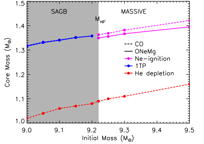
Figure 31. CO (dashed line) and ONeMg (solid line) core mass as a function of the initial mass at various evolutionary stages: core He depletion (red line and dots), first thermal pulse (blue line and dots), and Ne ignition (magenta line and dots).
