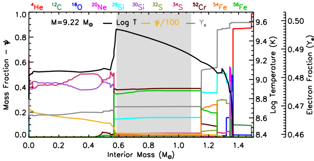
Figure 36. Selected chemical and physical properties (see the legend) of the 9.22 M_{\odot} star during the off-center Si-S burning.
