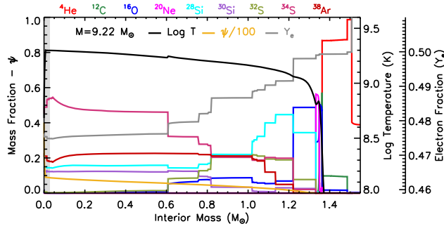
Figure 34. Selected chemical and physical properties (see the legend) of the 9.22 M_{\odot} (left panel) and 12.0 M_{\odot} models when the ONe burning front has reached the center.
