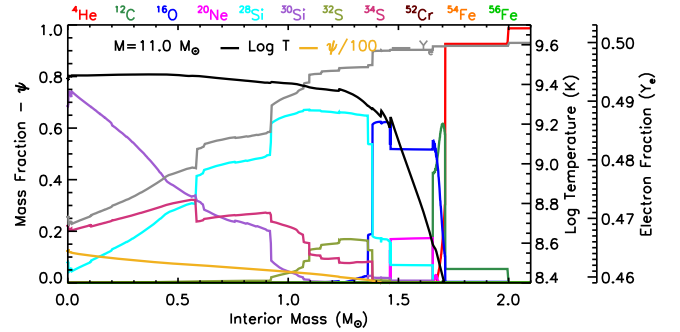
Figure 39. Selected chemical and physical properties (see the legend) of the 11.0 M_{\odot} model during the shell O-burning phase.
