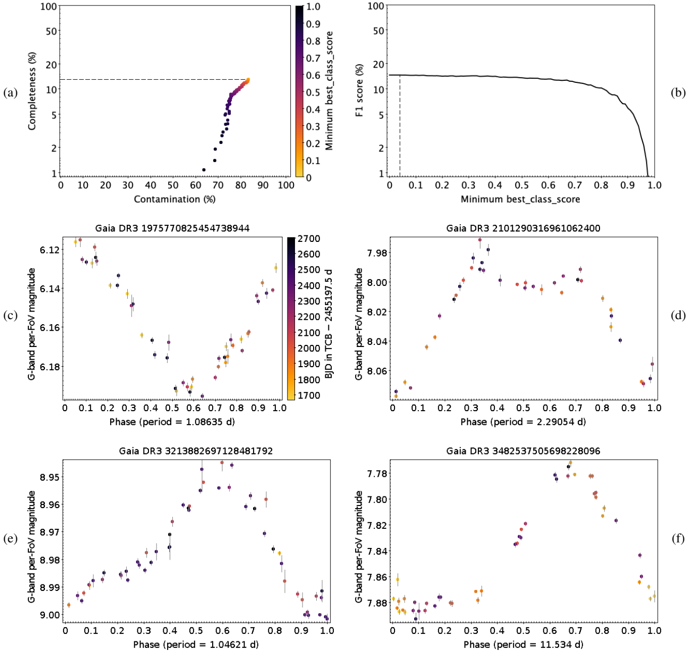
Fig. E.3. ACV|CP|MCP|ROAM|ROAP|SXARI: completeness, contamination, F_1 -score, and sample light curves. The dashed lines indicate the maximum completeness (with minimum best_class_score of zero) in panel (a) and the minimum best_class_score that maximises the F_1 -score (for an optimal balance between completeness and contamination) in panel (b). For all period-folded light curves, times are colour-coded according to the same legend as shown in panel (c).
