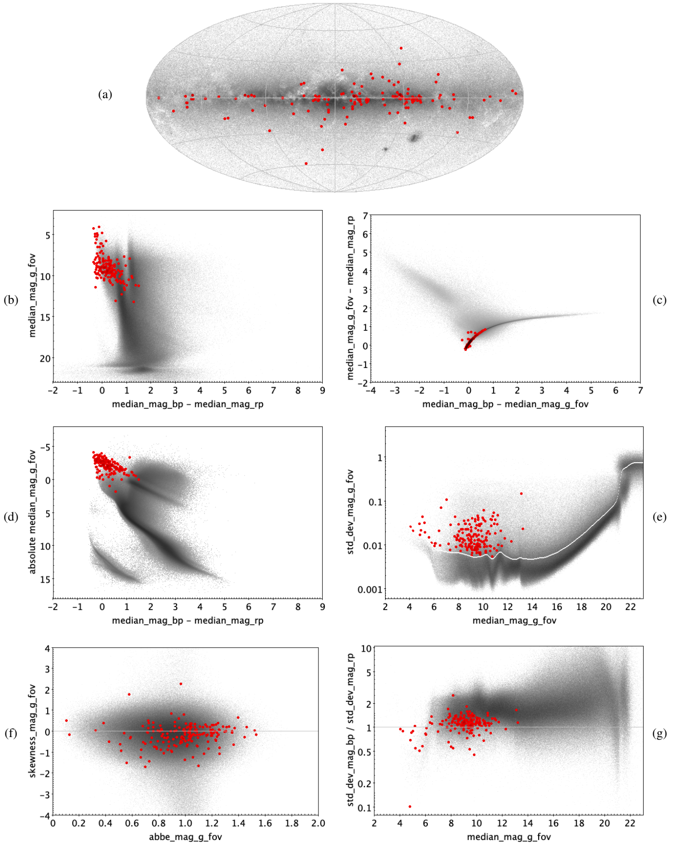
Fig. E.10. B CEP: 173 training sources.
