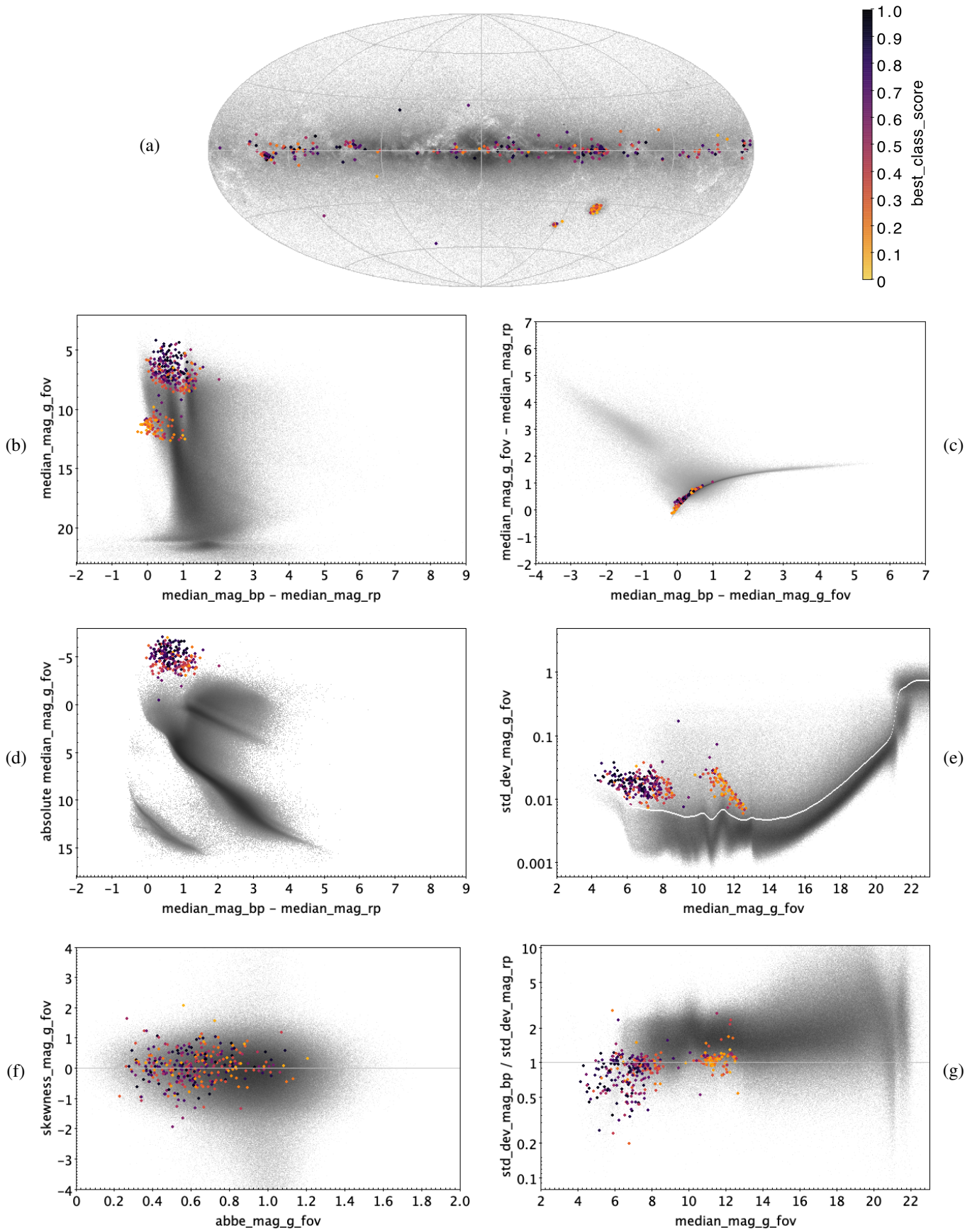
Fig. E.5. ACYG: 329 classified sources.
