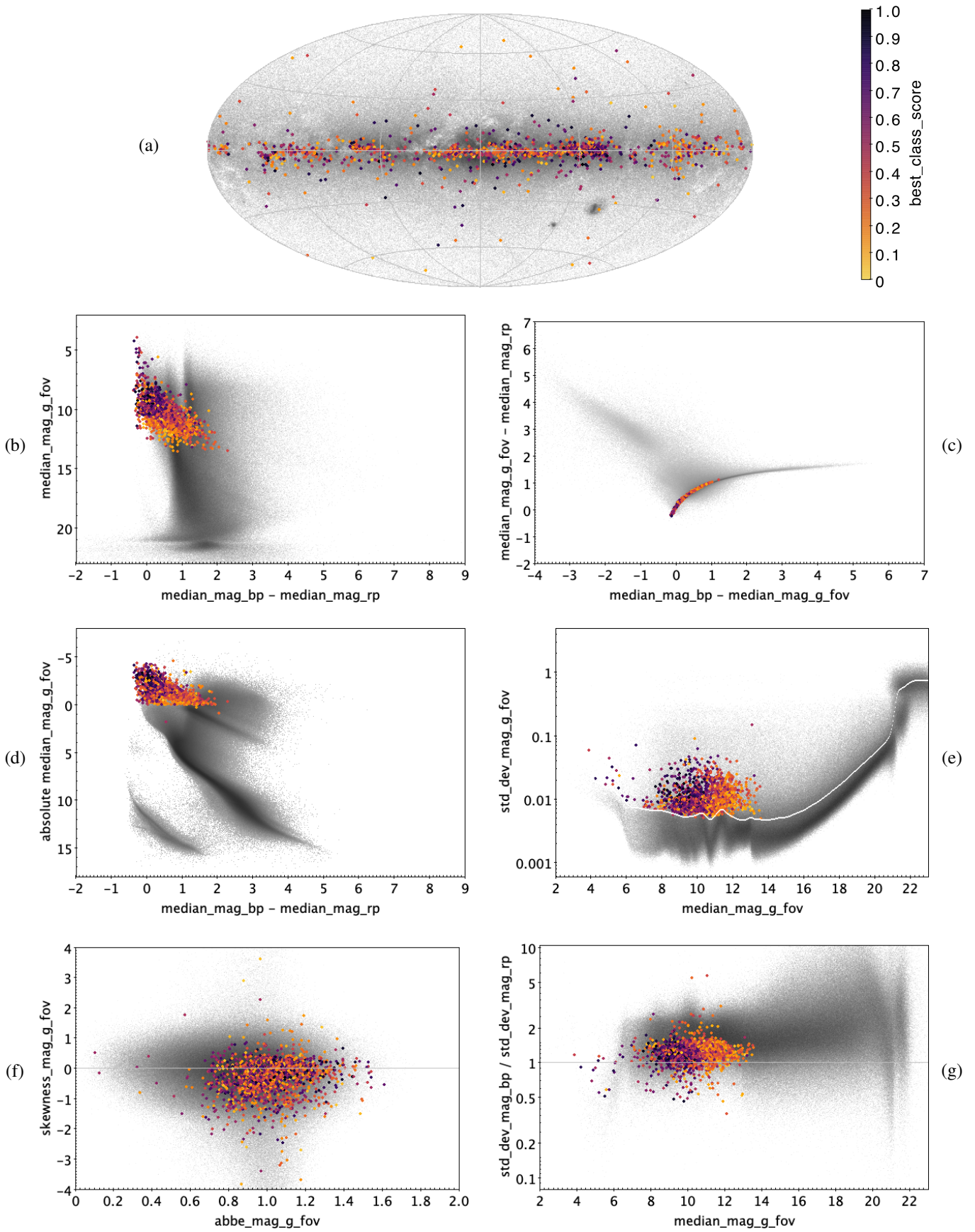
Fig. E.11. BCEP: 1475 classified sources.
