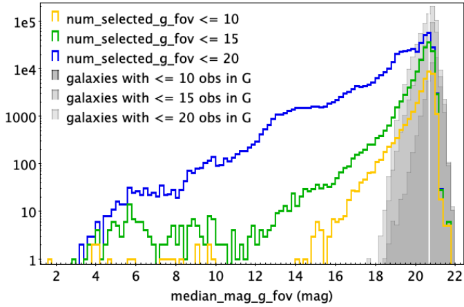
Fig. 2. Number of the least-sampled sources in 0.2 mag intervals as a function of the median G -band magnitude. The number of variable sources (in the vari_classifier_result table of the Gaia archive) is colour coded by the maximum number of selected FoV observations in the G band ( num_selected_g_fov up to 10, 15, and 20) as shown in the legend (with orange, green, and blue colours, respectively). The bars shaded in grey refer to the same conditions but for the galaxies identified by their artificial variability (published in the galaxy_candidates table), including unpublished values of num_selected_g_fov for galaxies outside the Gaia Andromeda Photometric Survey. The white vertical line marks the median G magnitude of 20.7. The fields num_selected_g_fov and median_mag_g_fov are published in the vari_summary table.
