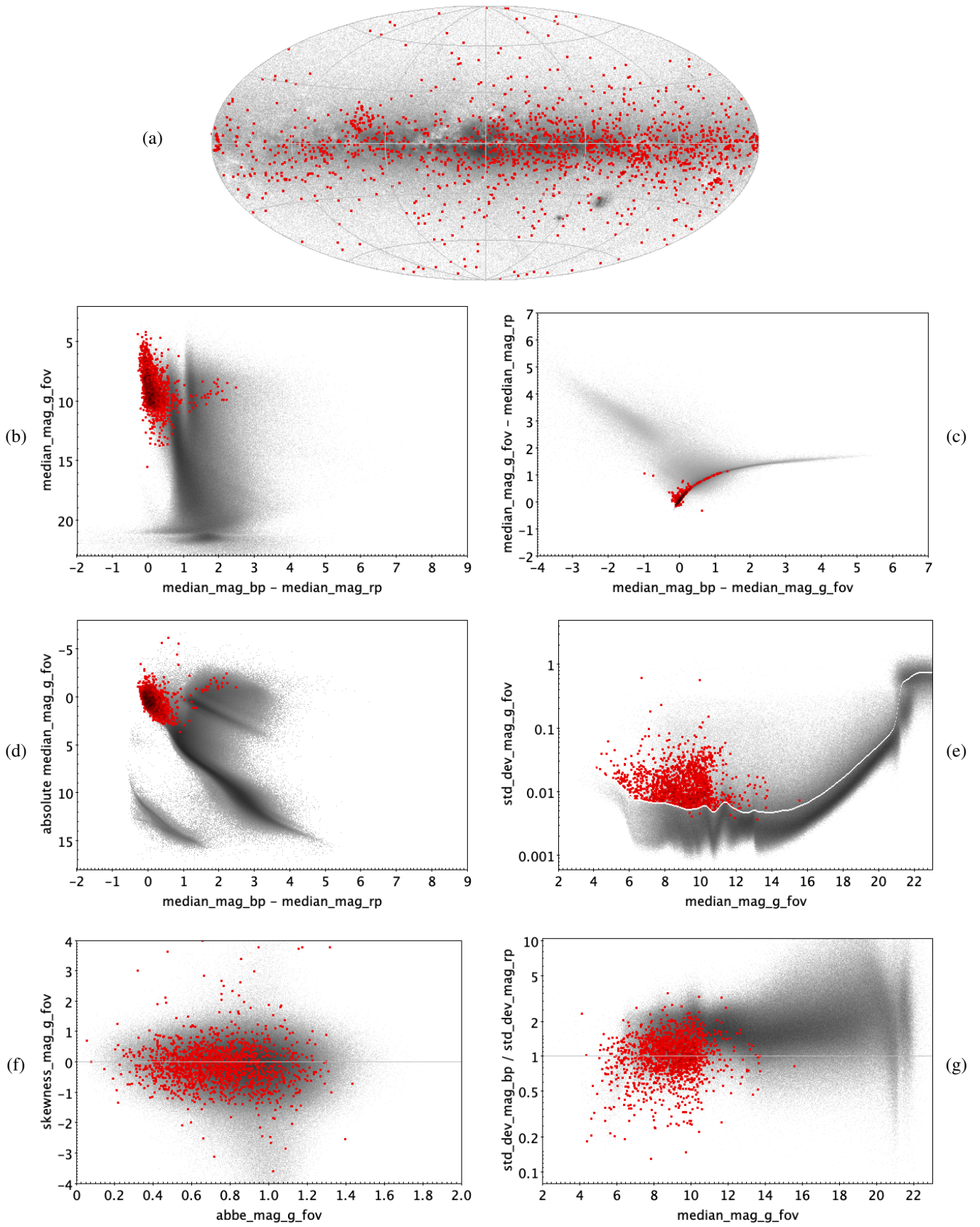
Fig. E.1. ACV|CP|MCP|ROAM|ROAP|SXARI: 1572 training sources.
