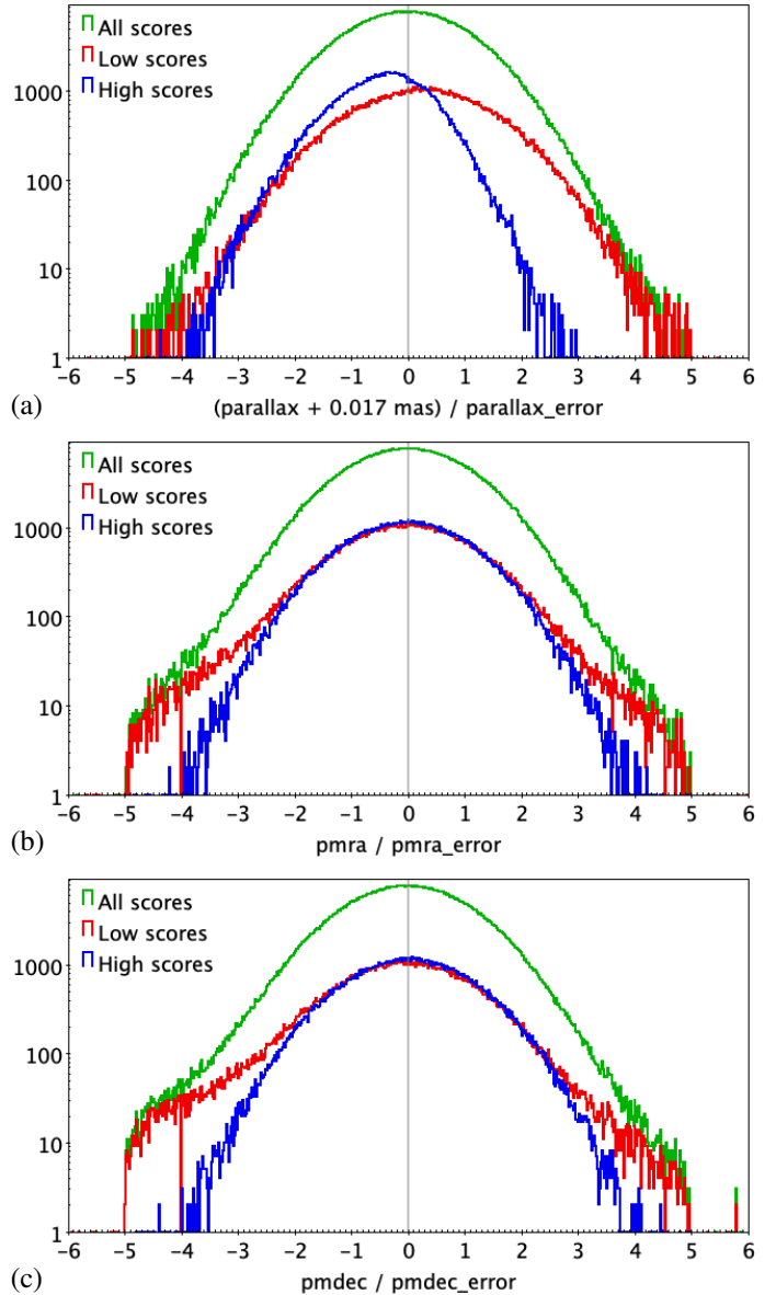
Fig. 4. Distribution of parallax (a) and proper motion components, pmra along the right ascension (b) and pmdec along the declination (c), normalised by the corresponding uncertainties and binned in intervals of 0.02, for the 1 034 925 AGN candidates with at least five-parameter astrometric solutions, for the top-150 000 candidates (denoted as high scores; best_class_score > 0.8995154), and for the bottom-150 000 candidates (denoted as low scores; best_class_score < 0.1615997), colour-coded as indicated in the legend. The bias from the inclusion of parallax among classification attributes is evident in panel a (see Sect. 4.3 for details).
