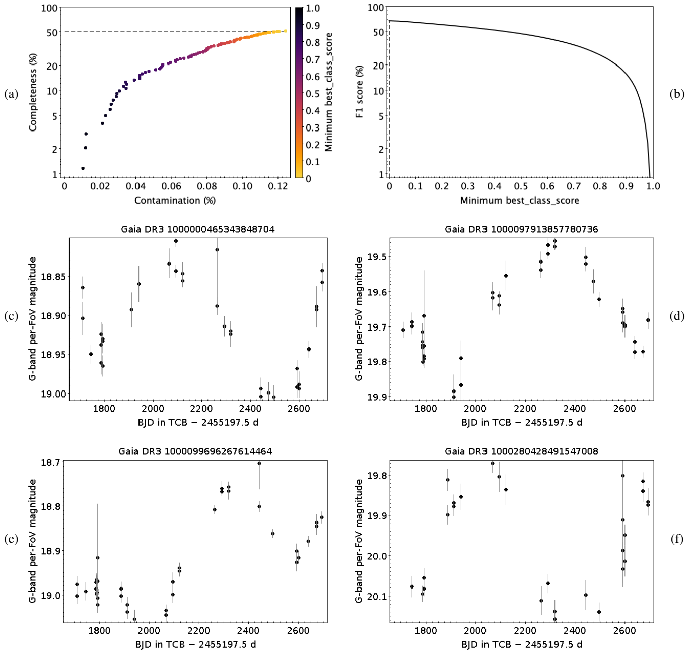
Fig. E.9. Same as Fig. E.3, but for AGN.
