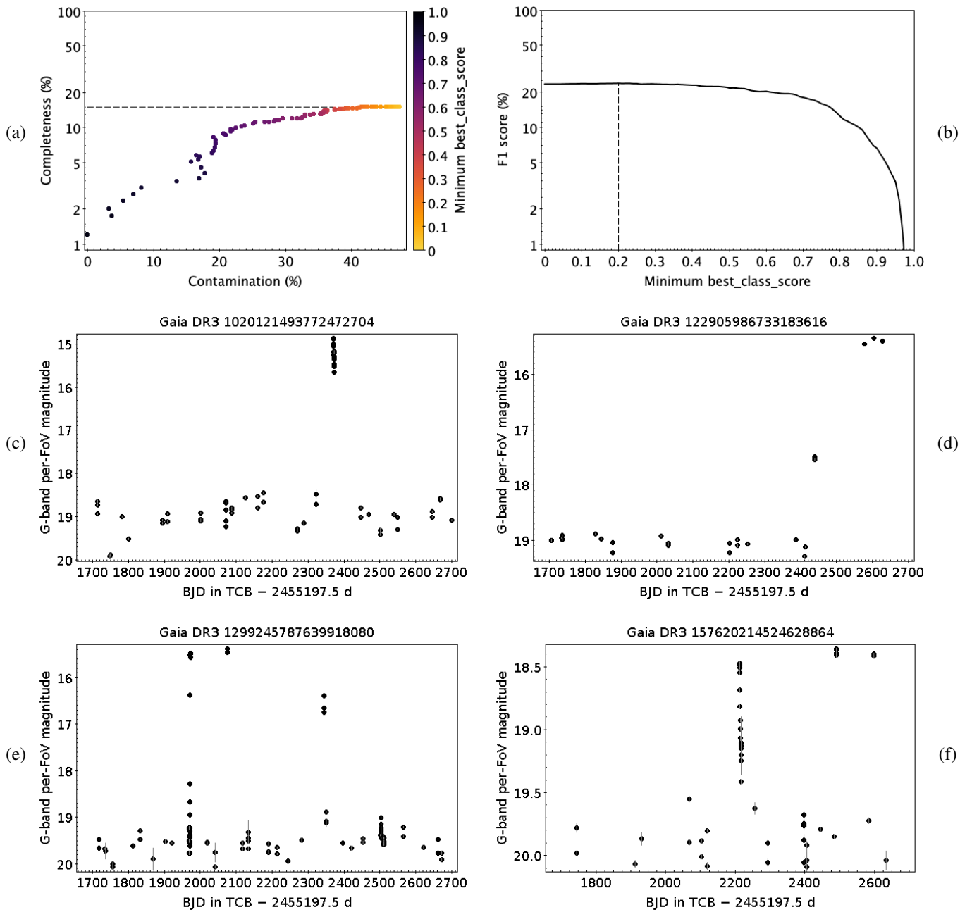
Fig. E.21. Same as Fig. E.3, but for CV.
