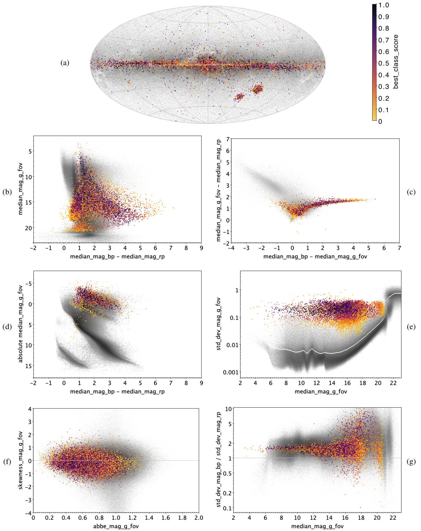
Fig. E.17. CEP: 16 141 classified sources.
