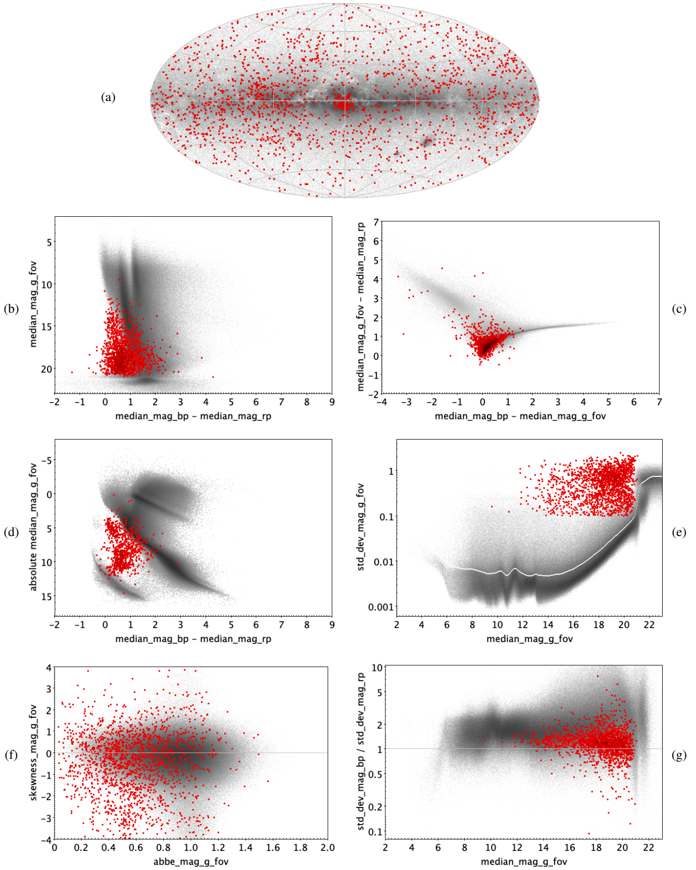
Fig. E.19. CV: 1815 training sources.
