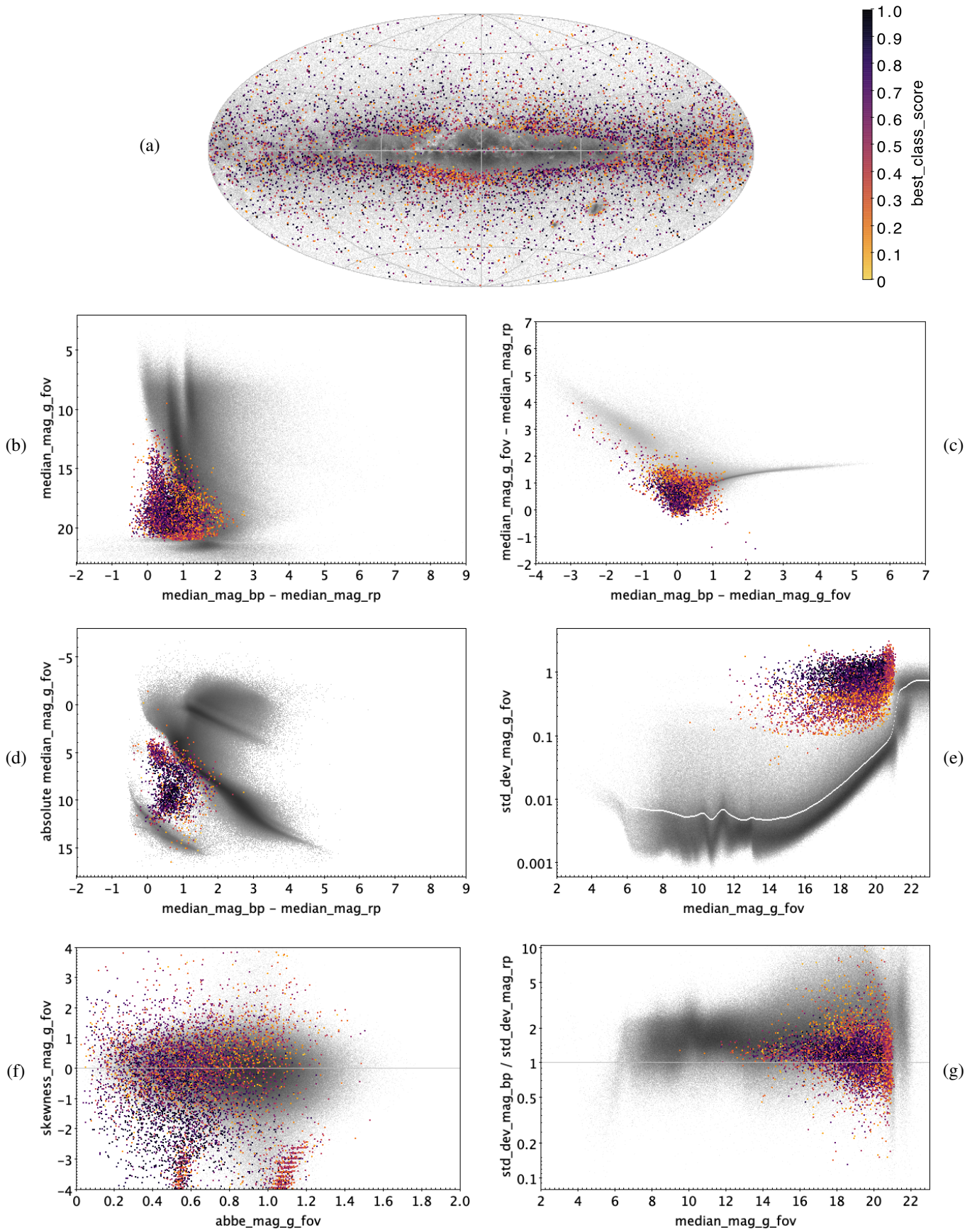
Fig. E.20. CV: 7306 classified sources.
