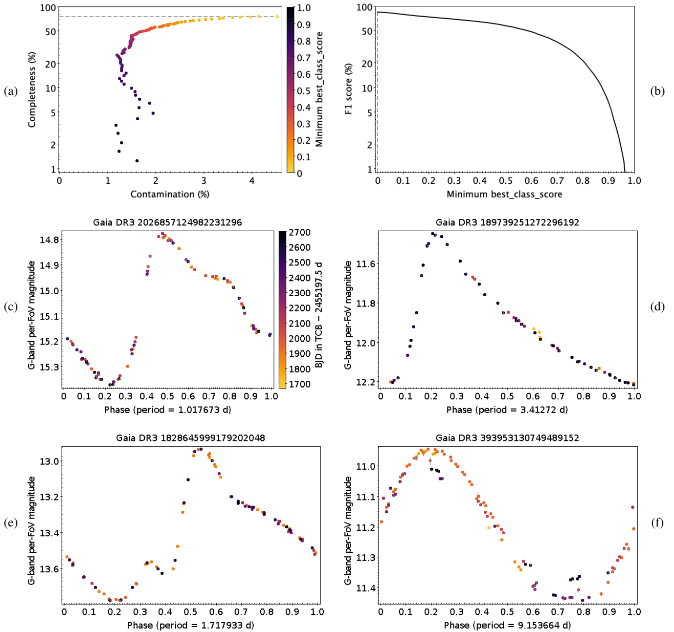
Fig. E.18. Same as Fig. E.3, but for CEP: (c) anomalous Cepheid, (d) \delta Cephei, (e) BL Herculis, and (f) W Virginis stars.
