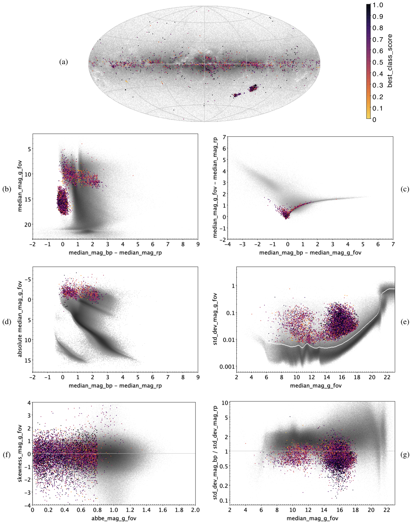
Fig. E.14. BE|GCAS|SDOR|WR: 8560 classified sources.
