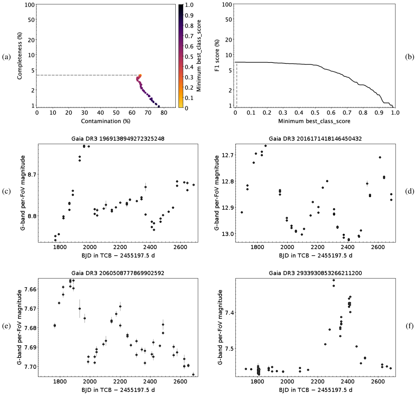
Fig. E.15. Same as Fig. E.3, but for BE|GCAS|SDOR|WR.
