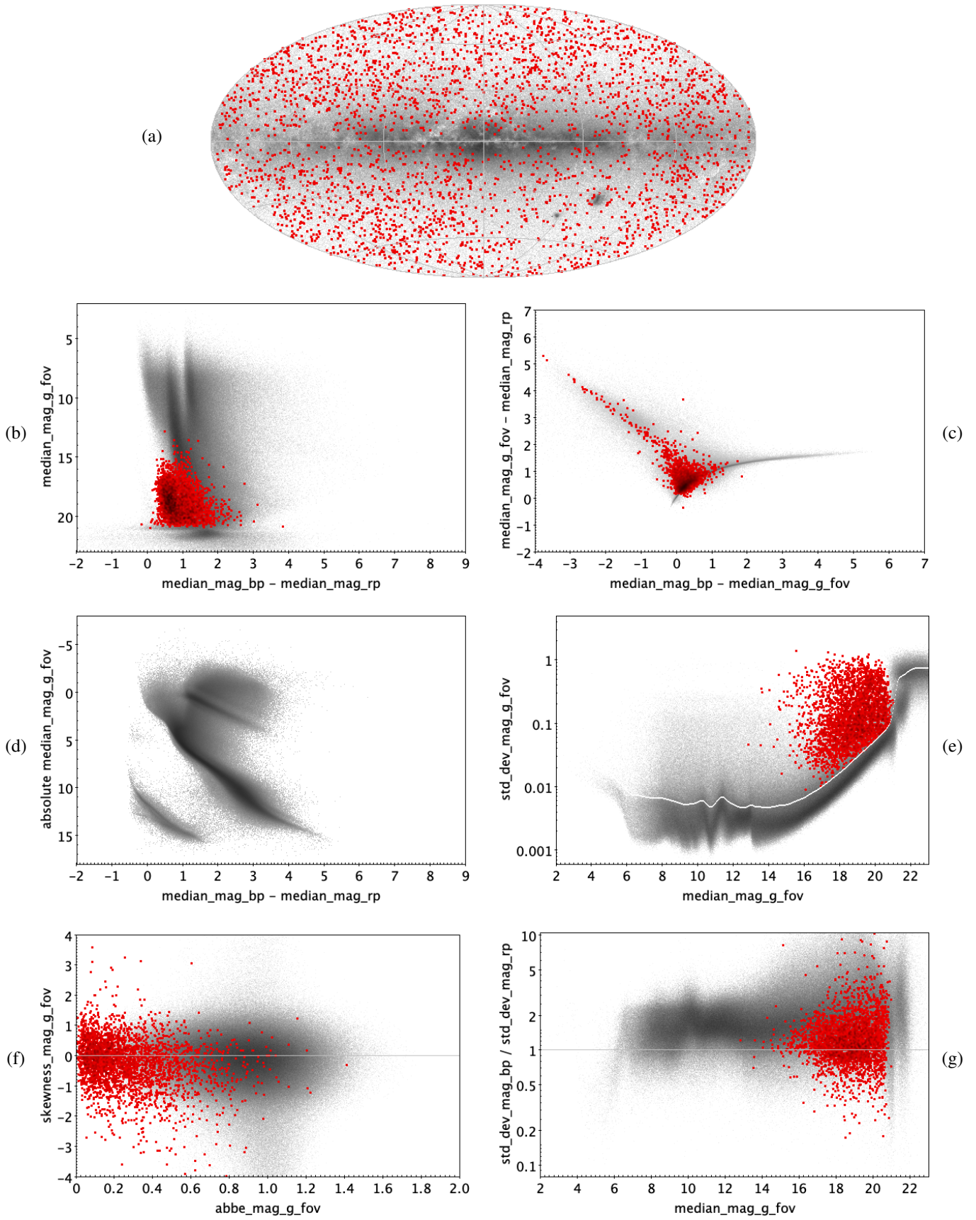
Fig. E.7. AGN: 3089 training sources.
