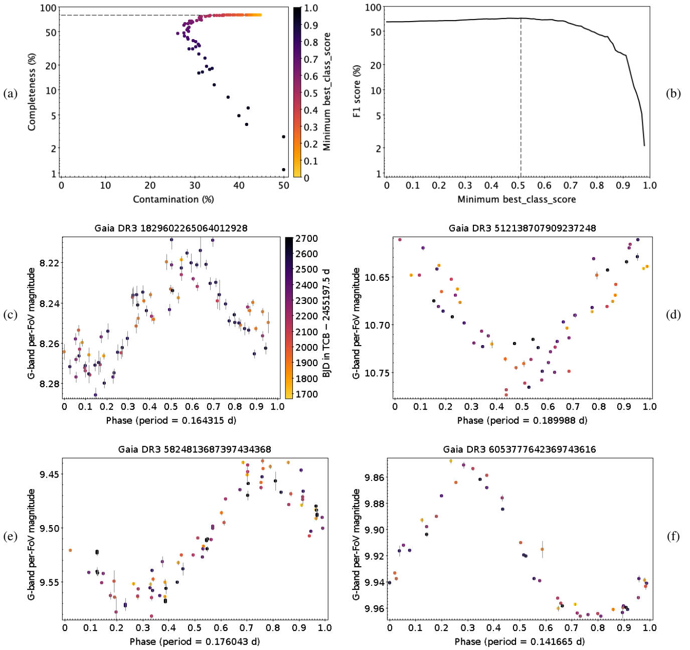
Fig. E.12. Same as Fig. E.3, but for BCEP.
