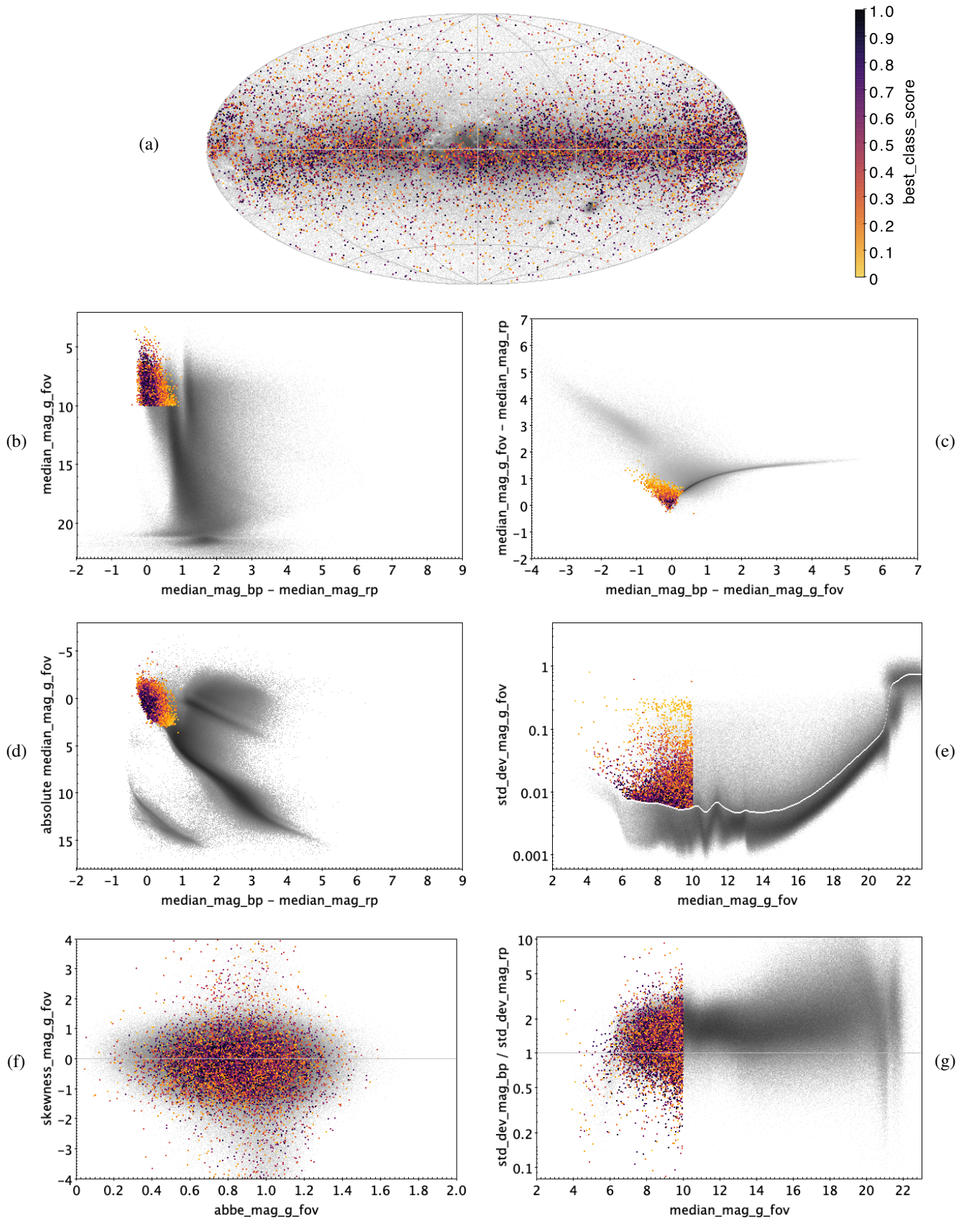
Fig. E.2. ACV|CP|MCP|ROAM|ROAP|SXARI: 10 779 classified sources.
