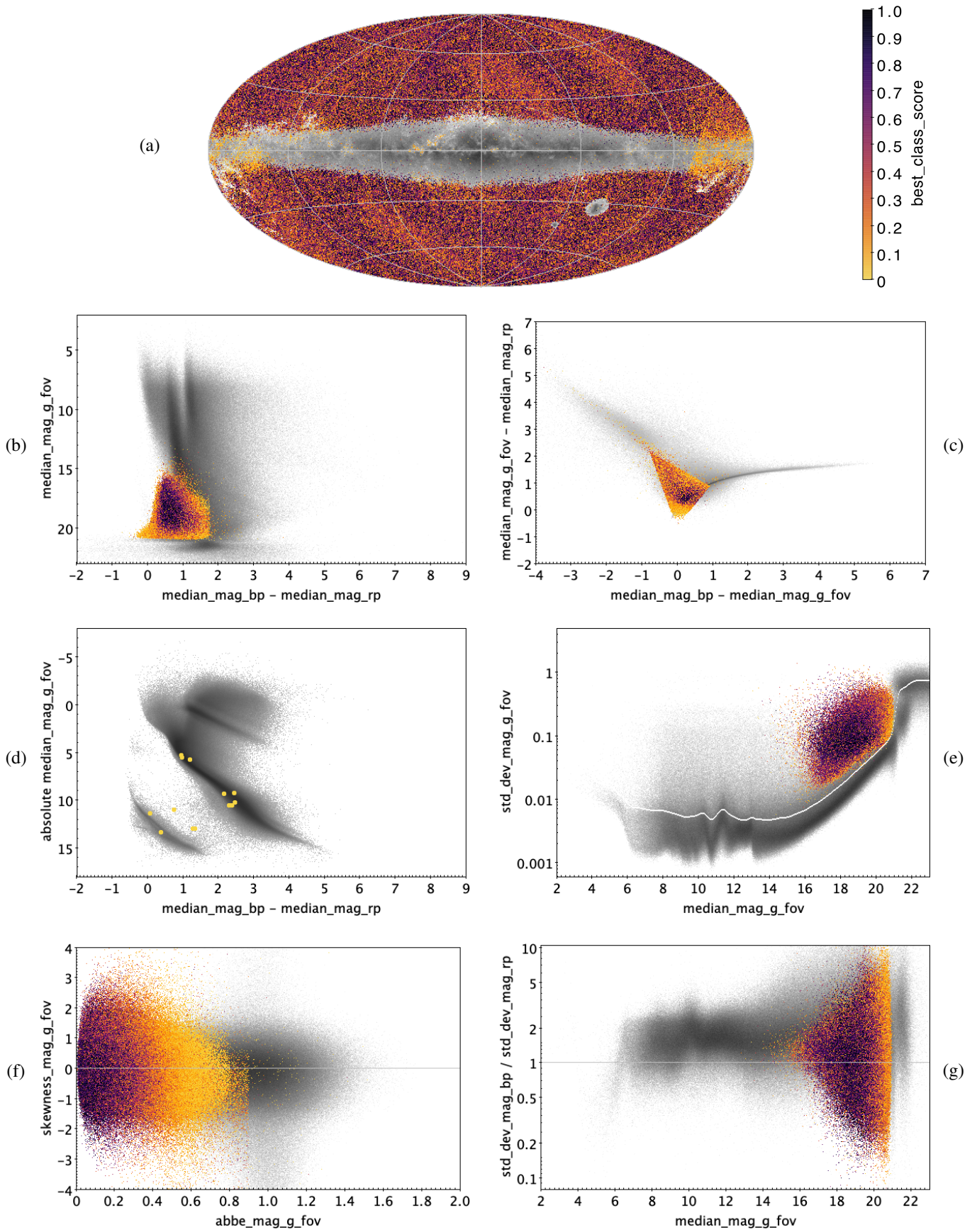
Fig. E.8. AGN: 1 035 207 classified sources.
