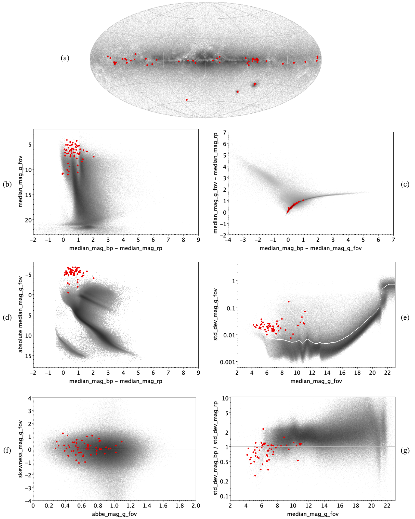
Fig. E.4. ACYG: 59 training sources.
