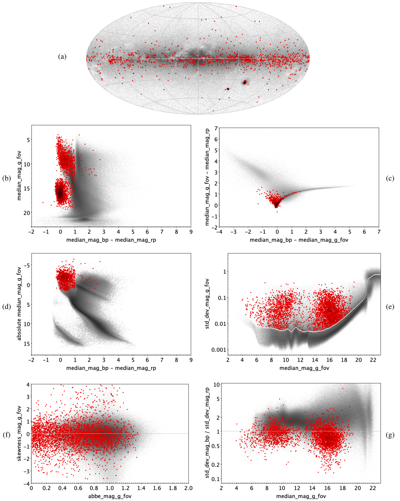
Fig. E.13. BE|GCAS|SDOR|WR: 3546 training sources.
