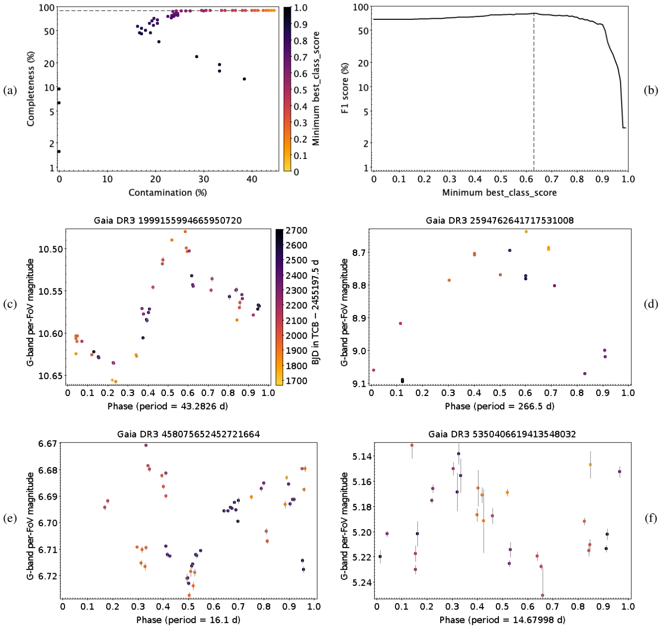
Fig. E.6. Same as Fig. E.3, but for ACYG.
