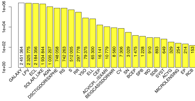
Fig. 1. Number of sources per class, sorted in decreasing order. The bars shaded in yellow correspond to variability types published in the vari_classifier_result table, while galaxies, identified by their artificial photometric variations in Gaia , are published exclusively in galaxy_candidates . The ACV|CP|MCP|ROAM|ROAP|SXARI class group is abbreviated as ACV|CP|...|SXARI.
