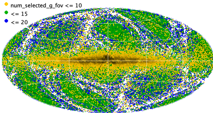
Fig. 3. Sky map of the least-sampled sources in Galactic coordinates (white grid), colour coded as in Fig. 2 for variable sources with num_selected_g_fov up to 10, 15, and 20. Galactic longitude is zero at the centre and increases towards the left. The thin line in black denotes the Ecliptic.
