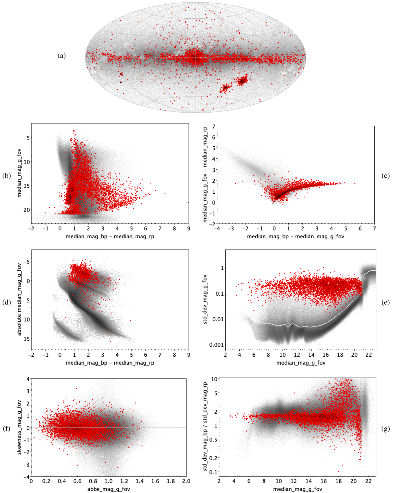
Fig. E.16. CEP: 4448 training sources.
