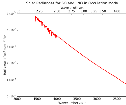
Fig. 3. Solar spectral radiance entering the SO and LNO solar occultation apertures. Note that radiance is invariant with Sun-Mars distance. Below 2.5\mu m solar absorption lines are present in the spectrum.
