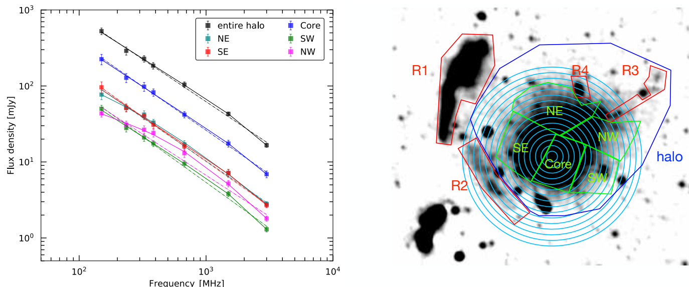
Fig. 6. Left: Integrated radio spectra of the entire halo and its subregions. The solid and dash-dotted lines show fitted power-law and double power-law spectra, respectively. The radio spectrum of the halo is described by a power-law between 150 MHz and 3 GHz. Unlike the entire halo, its subregions show different spectra also featuring high frequency spectral steepening. Right: The flux density of the entire halo was extracted from the blue region, labeled as halo. Green regions were used to extract the flux density from the halo subregions. The blue annuli are used to compute the radio and X-ray surface brightness profiles. These annuli have widths of 15'' , similar to the radio beam size.
