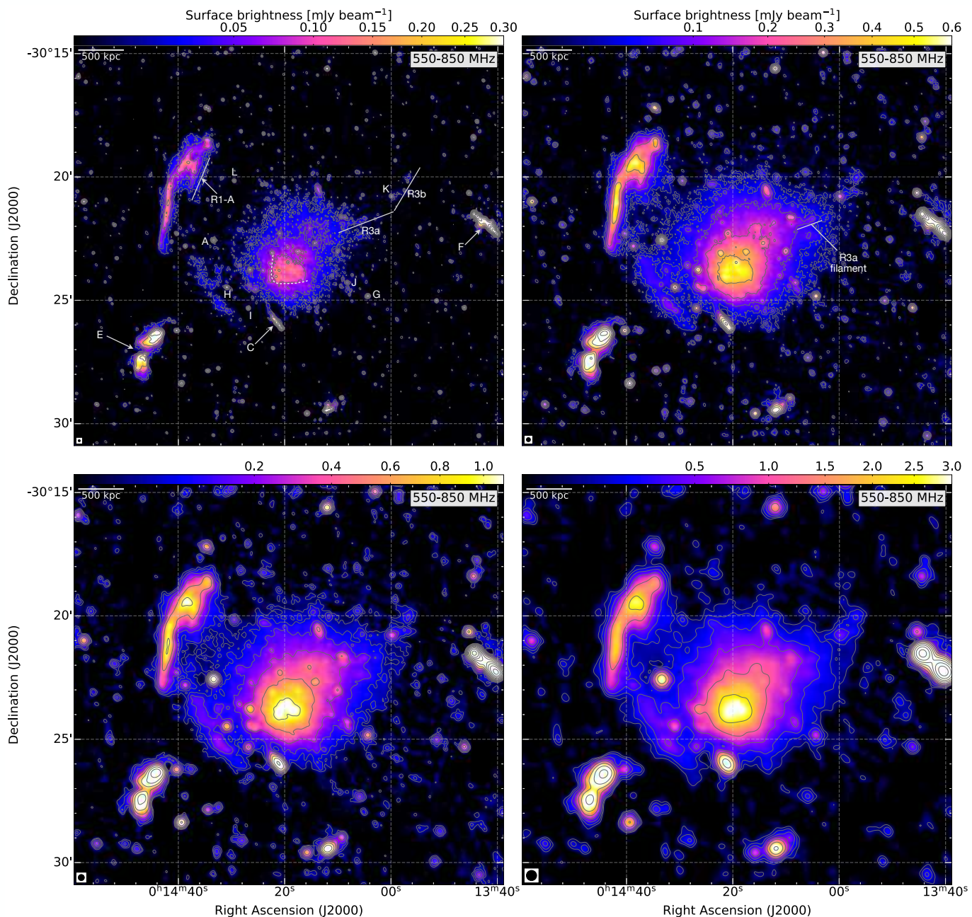
Fig. 3. Total power uGMRT (550-850 MHz) images of Abell 2744 at different resolutions ( 5'' , top left; 10'' , top right; 15'' , bottom left; 25'' , bottom right). The known diffuse emission sources, namely the main relic (R1), the fainter relics (R2, R3, and R4), and the extended halo are recovered in our new uGMRT observations. The radio emission at the center of the halo apparently shows a cone-like morphology. The image properties are given in Table 2. Here, panel top left, top right, bottom left and bottom right correspond to IM9, IM10, IM12, and IM15, respectively. Contour levels are drawn at [1, 2, 4, 8, \dots] \times 3.5 \sigma_{\text{rms}} . In these images there is no region below -3 \sigma_{\text{rms}} . The beam size is indicated in the bottom left corner of the each image.
