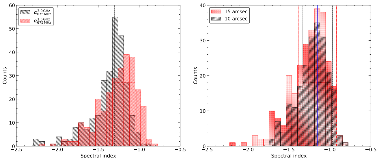
Fig. 10. Left: Histogram of the spectral index distribution across the halo in Abell 2744 for different sets of frequencies. The low frequency values were obtained between 675 MHz and 1.5 GHz (in red) while the other one between 675 MHz and 3 GHz (in black). The spectral indices were extracted from 15'' boxes, corresponding to a physical size of about 67 kpc. The dashed lines represent the median spectral index values. Right: Histogram of spectral index values obtained from 10'' (black) and 15'' (red) resolution radio maps created between 675 MHz and 1.5 GHz. The plot suggest that the distribution of the mean spectral index and its standard deviation have a little impact when adopting different resolutions. The solid blue line represents the median value, \langle\alpha\rangle = -1.15 , at both 10'' and 15'' resolution. The dash-dotted (red) and dashed (black) lines represent the standard deviation around the median values at 10'' ( \sigma_{10''} = 0.19 ) and 15'' ( \sigma_{15''} = 0.24 ), respectively.
