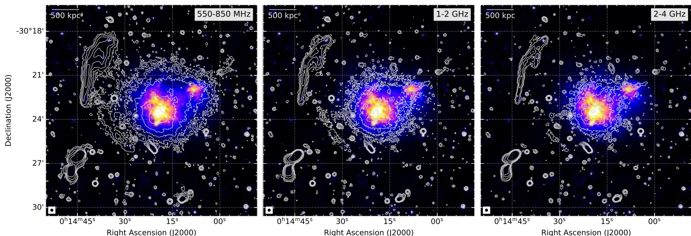
Fig. 5. Chandra (0.5 – 2.0 keV band) X-ray image overlaid with radio contours at 675 MHz, 1.5 GHz, and 3.0 GHz. All radio images are created at a common resolution of 10'' . Here, left, middle, and right panels correspond to IM10, IM5, and IM1, respectively. The halo emission is apparently more extended toward low frequencies, in particular to the northeast direction. Contour levels are drawn at [1, 2, 4, 8, \dots] \times 3.5 \sigma_{\text{rms}} . In all three images there is no region below -3.0 \sigma_{\text{rms}} . The beam size is indicated in the bottom left corner of the each image.
