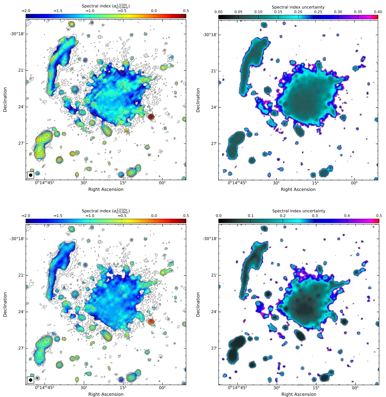
Fig. 9. Left: Spectral index maps of the halo between 675 MHz and 1.5 GHz (top) and 675 MHz and 3.0 GHz (bottom) at 15'' resolution. The image properties are given in Table 2, IM3, IM7, and IM13. Contour levels are drawn at [1, 2, 4, 8, \dots] \times 3.5 \sigma_{\text{rms}} , and are from the uGMRT Band 4 image. These maps show the presence of steeper spectral indices in outermost regions of the halo, in particular to the north. Right: Corresponding spectral index uncertainty.
