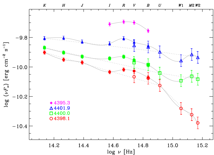
Fig. 5. Spectral energy distributions (SEDs) of 0716+714 in late October 2007, constructed with W2 M2 W1 U B V data from Swift-UVOT (empty symbols) and ground-based GASP-WEBT BVRJHK data (filled symbols). The numbers in the legend refer to the Julian Dates of the observations. The dotted lines connect the K , U , and W2 data; together with the cubic splines through the spectra, they help to better distinguish the main features of the SEDs (see text).
