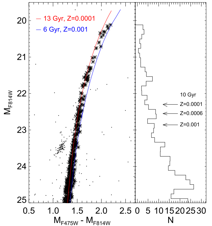
Figure 7. Left: CMD of And XVI showing the RGB stars (asterisks) used to detect the RGB tip. Two isochrones are also overplotted: Z = 0.0001 , t = 13 Gyr (red line), and Z = 0.001 , t = 6 Gyr (blue line). We assumed (m - M)_0 = 23.72 mag and E(B - V) = 0.06 mag. Right: luminosity function of RGB stars. The three arrows mark the expected position of the RGB bump for three isochrones of 10 Gyr: Z = 0.0001 , Z = 0.0006 , and Z = 0.001 .
