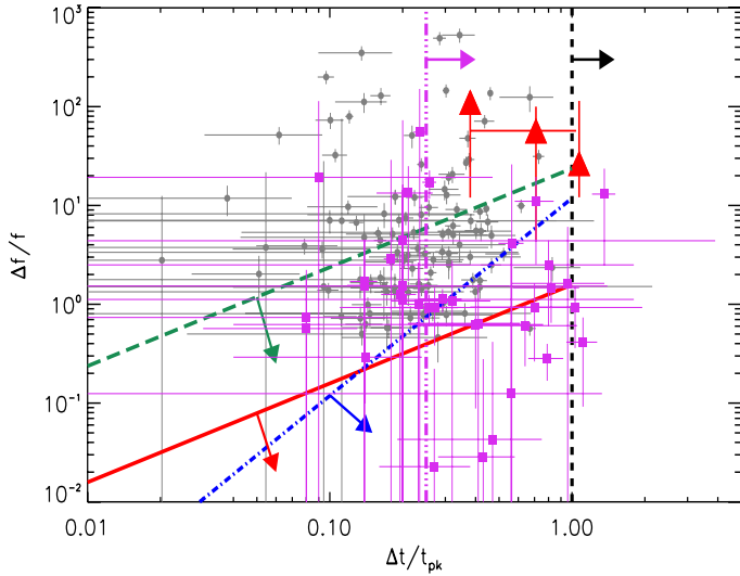
Fig. 7. Kinematically allowed regions for afterglow variability in the \Delta f/f vs. \Delta t/t_{pk} plane. Coloured lines with arrows represent the permitted regions for density fluctuations on-axis (blue), density fluctuations off-axis (red), multiple density fluctuations off-axis (green), refreshed shocks (pink), and patchy shell (black). (See Ioka et al. 2005; Chincarini et al. 2010; Bernardini et al. 2011, for details.) In this plot we show early-time ( t_{pk} \lesssim 1 ks, grey points) and late-time ( t_{pk} \gtrsim 1 ks, magenta squares) flares. The red triangles are the three flaring episodes in GRB 140515A. The error bars account for the uncertainty on the behaviour of the underlying continuum: the lower bar corresponds to a flat power-law decay after 10^3 s, the high bar to a flat decay normalised to the last datapoint, and the central value to a power-law decay consistent with the slope of the optical light curve after 10^3 s.
