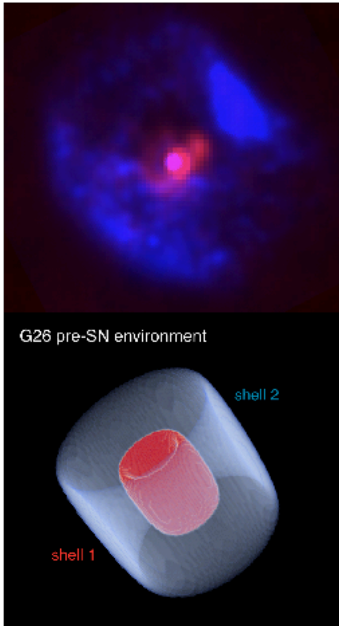
Fig. 2. Top: map of G26 which combines infrared at 24\ \mu\text{m} (blue) and radio (red) images (see Umama et al. 2012). Bottom: schematic view of the CSM around G26, representing the two dense shells (in red and light blue) observed in the radio and infrared bands. The LBV is located in the center of the two nested toroidal shells.
