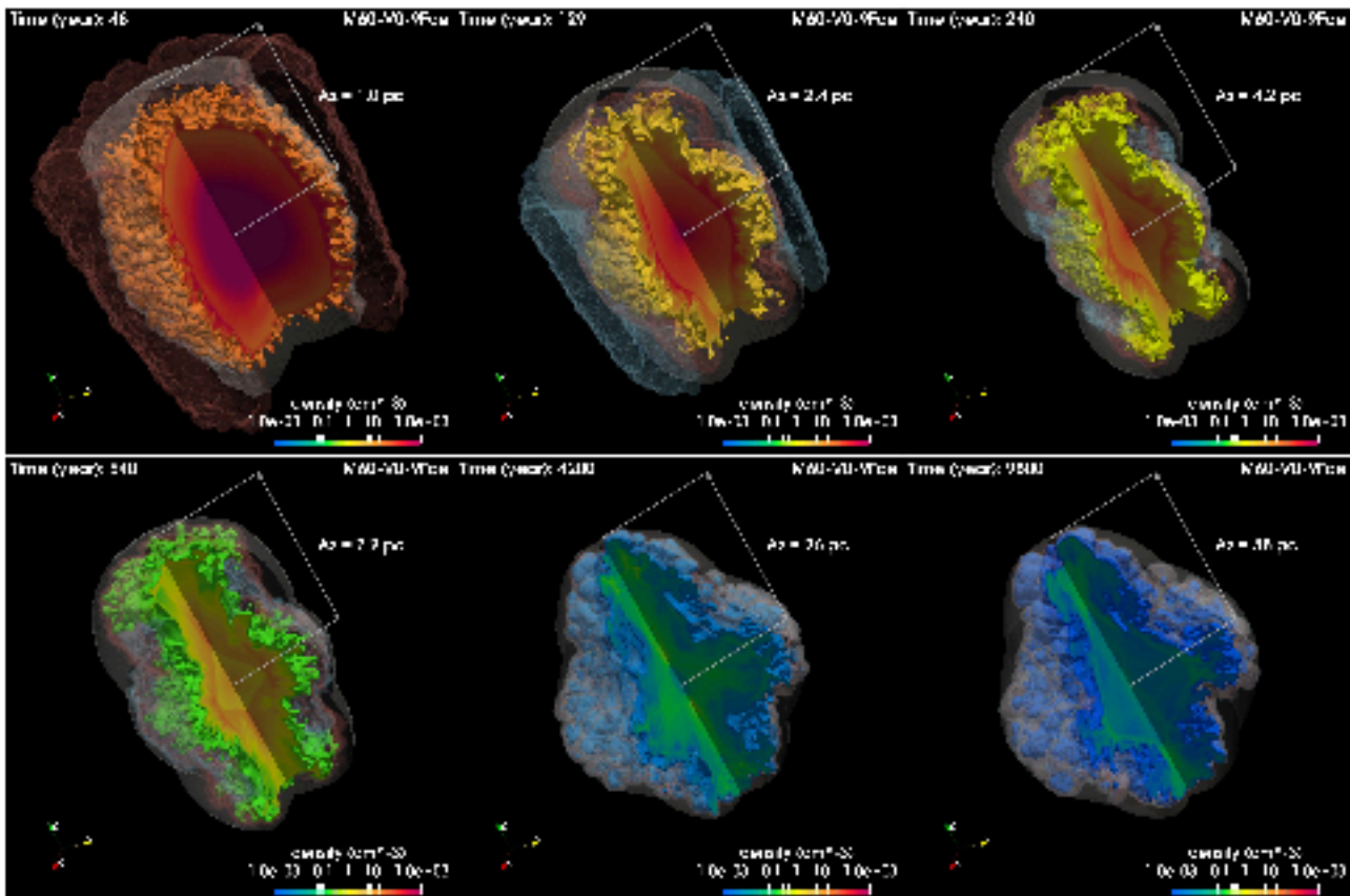
Fig. 5. Same as in Fig. 3 but for model M60-V0-9Fov. The complete temporal evolution is available online (Movie 3).
