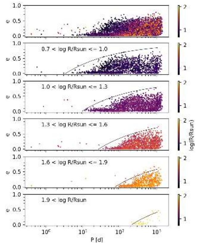
Fig. 24. e – P diagram for SB1 systems along the giant branch, filtered according to significance factors larger than 40, for various radius spans. Top panel: is the full sample. The solid black lines correspond to the loci where P(1 - e)^3 is constant (see text). The sample sizes are, from top to bottom, 1960, 2358, 1643, 737, and 40. The location in the HRD of the SB1 systems with 0.7 < \log(R/R_{\odot}) \leq 1.0 ( second panel from top ), 1.3 < \log(R/R_{\odot}) \leq 1.6 ( fourth panel from top ) and 1.9 < \log(R/R_{\odot}) ( bottom panel ) is shown in Fig. 25.
