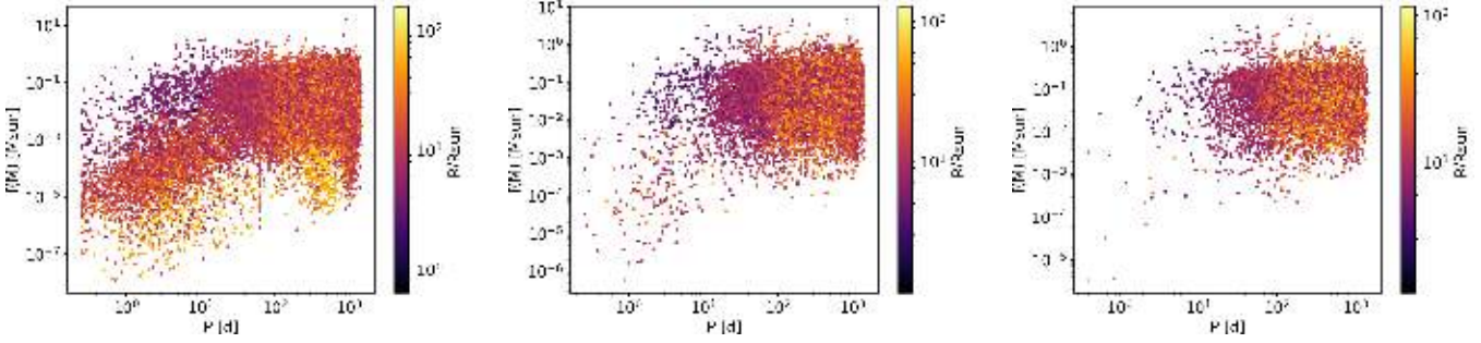
Fig. 23. P – f(M) diagrams for SB1 along the RGB/AGB. Left (a): unfiltered. The yellow tail extending down to f(M) \sim 10^{-5} M_{\odot} at periods in the range 300–800 d corresponds to pseudo-orbits associated to long-period pulsators (see Sect. 6.2.3). Middle (b): filtered by significance >20 and >40 ( right (c) ).
