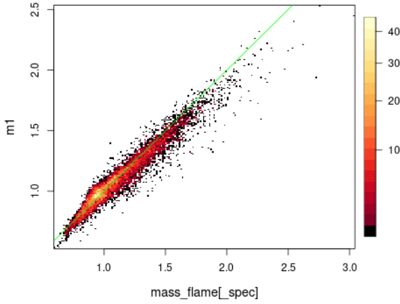
Fig. E.1. Density plot of the comparison between the primary masses derived here with the FLAME ones for systems with fluxratio < 0.01.
