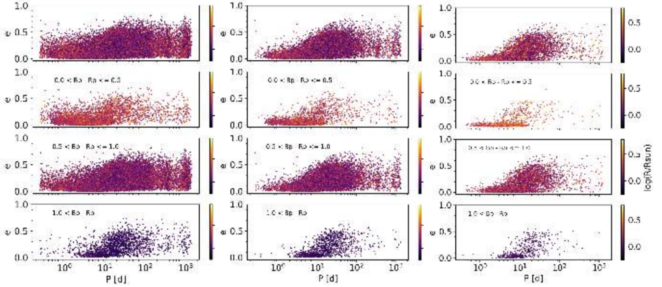
Fig. 20. The e – P diagram for SB1s along the main sequence, filtered according to significance factors larger than 10, 20, or 40 (from left to right), and for different (G_{BP,0} - G_{RP,0}) spans (top to bottom). Filtering on the significance removes potentially spurious high-eccentricity solutions at small periods with the side effect of removing long period solutions. The drop in the number of systems at P = 0.5 yr due to insufficient sampling at this specific period. The color codes for the FLAME radius estimate.
