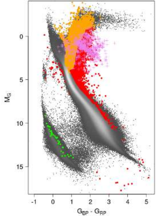
Fig. E.2. HRD of the NSS astrometric solutions without a primary mass estimate. The grey background is the HRD of the full DR3 low-extinction stars ( A_0 < 0.05 according to Lallement et al. 2019 ), equivalent to Fig. 5 of Gaia Collaboration (2018a) . The orange points are identified as giants. The red points do not have isochrone match. Violet + do not have an extinction estimate and uncorrected magnitude and colour are therefore used for those. Green points are the white dwarfs with a mass of 0.65 \pm 0.16 M_\odot assumed for Table 3.
