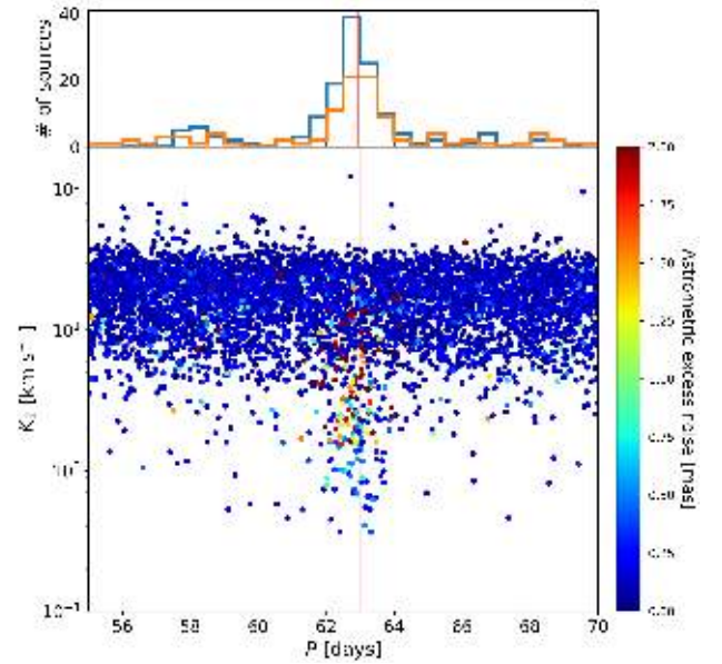
Fig. 5. K_1 semi-amplitude vs. period diagram of SB1 solutions, colour coded according to their astrometric_excess_noise . The diagram shows the presence of an overdensity of solutions at periods near the precession period (marked with a vertical line) with large astrometric excess noise. The histogram at the top shows the density of solutions with astrometric excess noise larger than 1 mas (blue line) and of those with ipd_frac_multi_peak > 20 (orange line).
