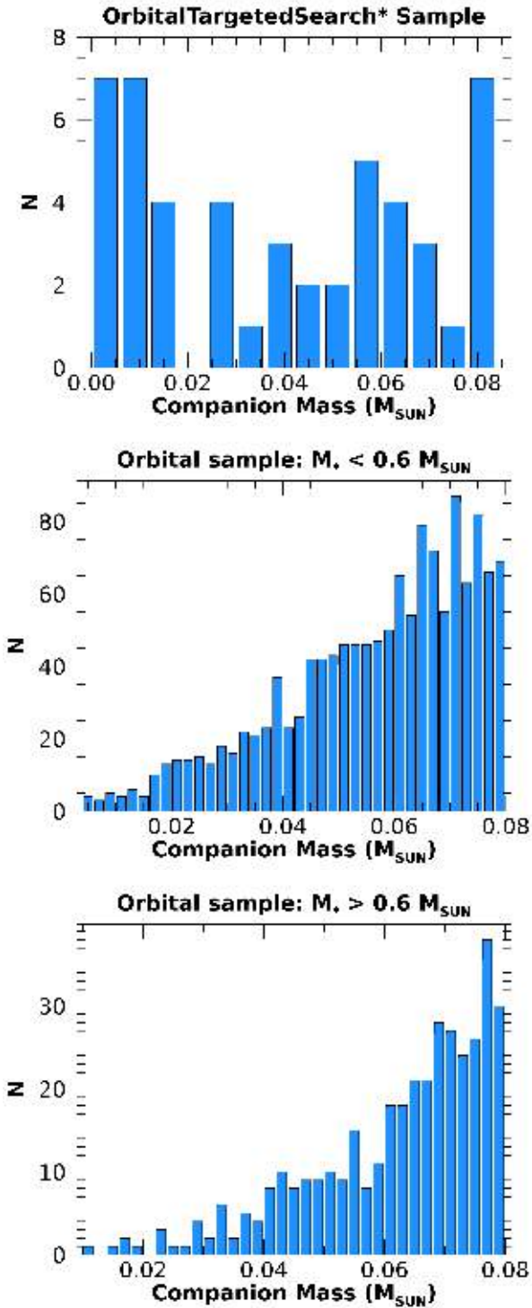
Fig. 49. Top: substellar companion mass distribution for the OrbitalTargetedSearch* solution type. Centre: same as above, but for the Orbital solution type, with a cut-off in the primary mass M_1 < 0.6 M_{\odot} . Bottom: same again, but for the Orbital solution type, with a cut-off in the primary mass M_1 > 0.6 M_{\odot} .
