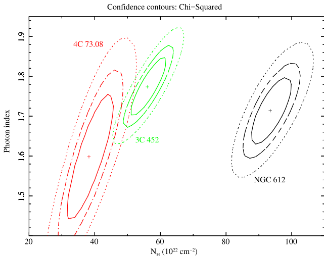
Figure 3. Contour plots of the column density N_{\text{H}} versus the photon index of the primary power law (MYTORUS model, see Table 3) for NGC 612 (black), 4C 73.08 (red) and 3C 452 (green). Solid, dashed and dotted lines correspond to 68 per cent, 90 per cent and 99 per cent confidence levels, respectively.
